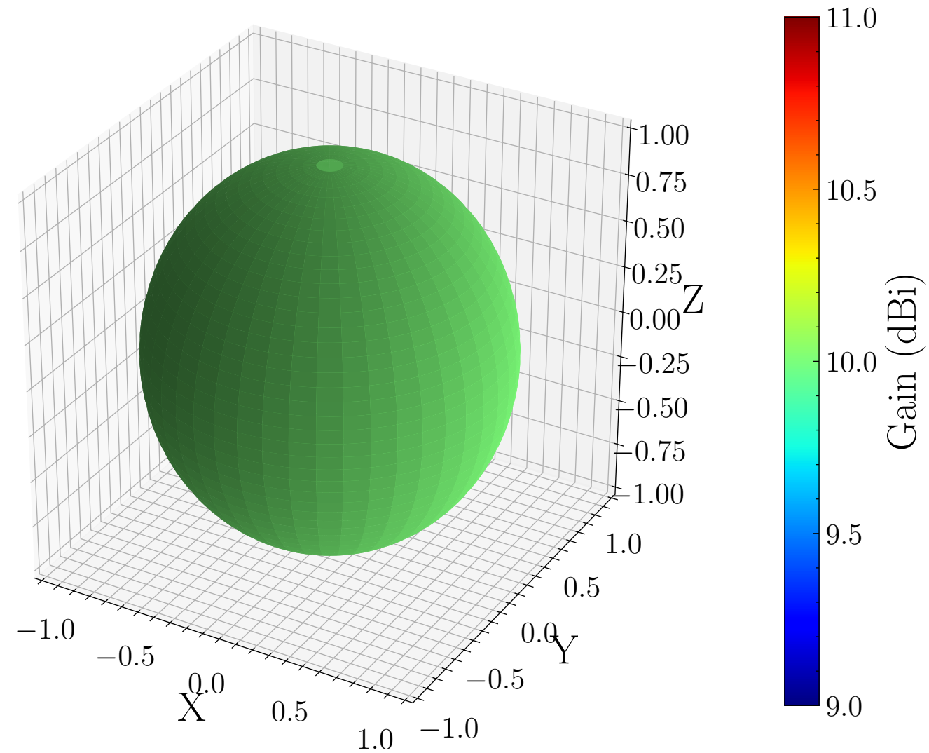
3D Pattern (Estimated from H/V)
