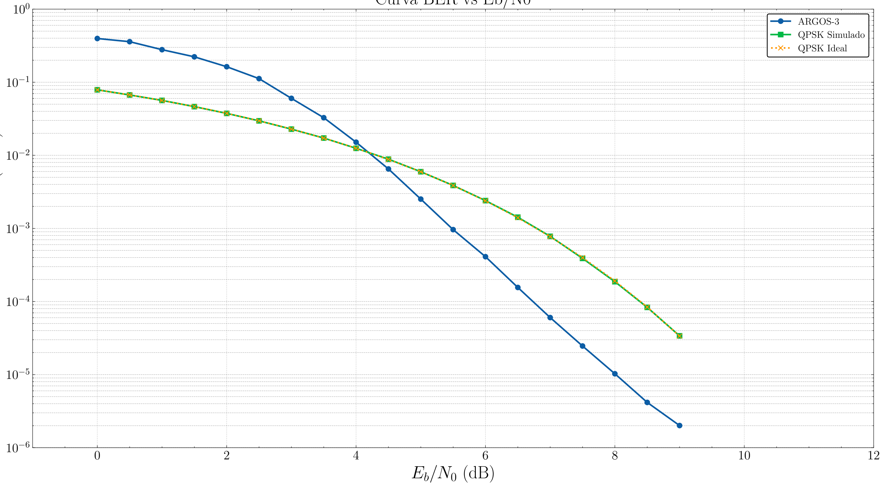
Curva BER vs Eb/N0
