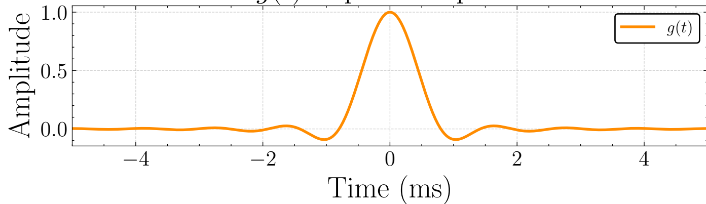
RRC Pulse Modulation
