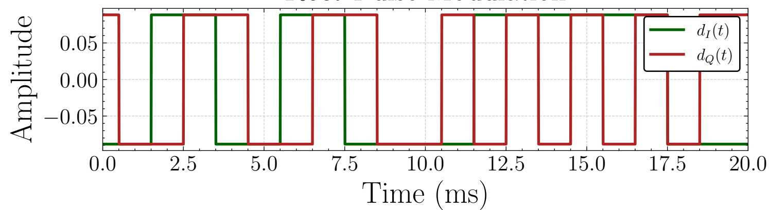
Rect Pulse Modulation
