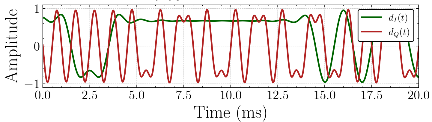
RRC Pulse Modulation
