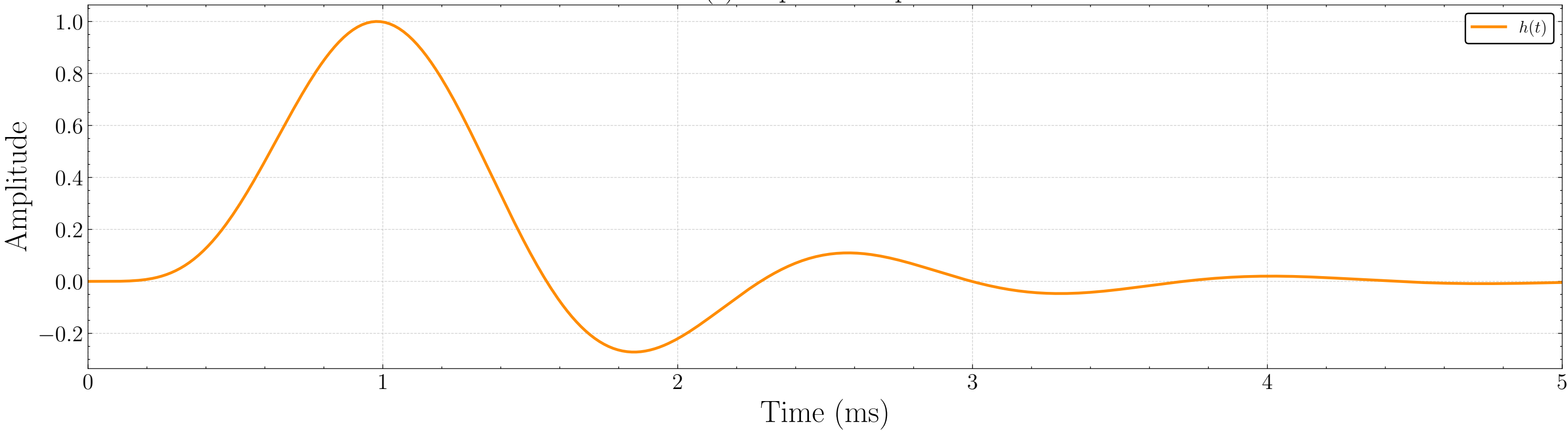
h(t) Impulse Response
