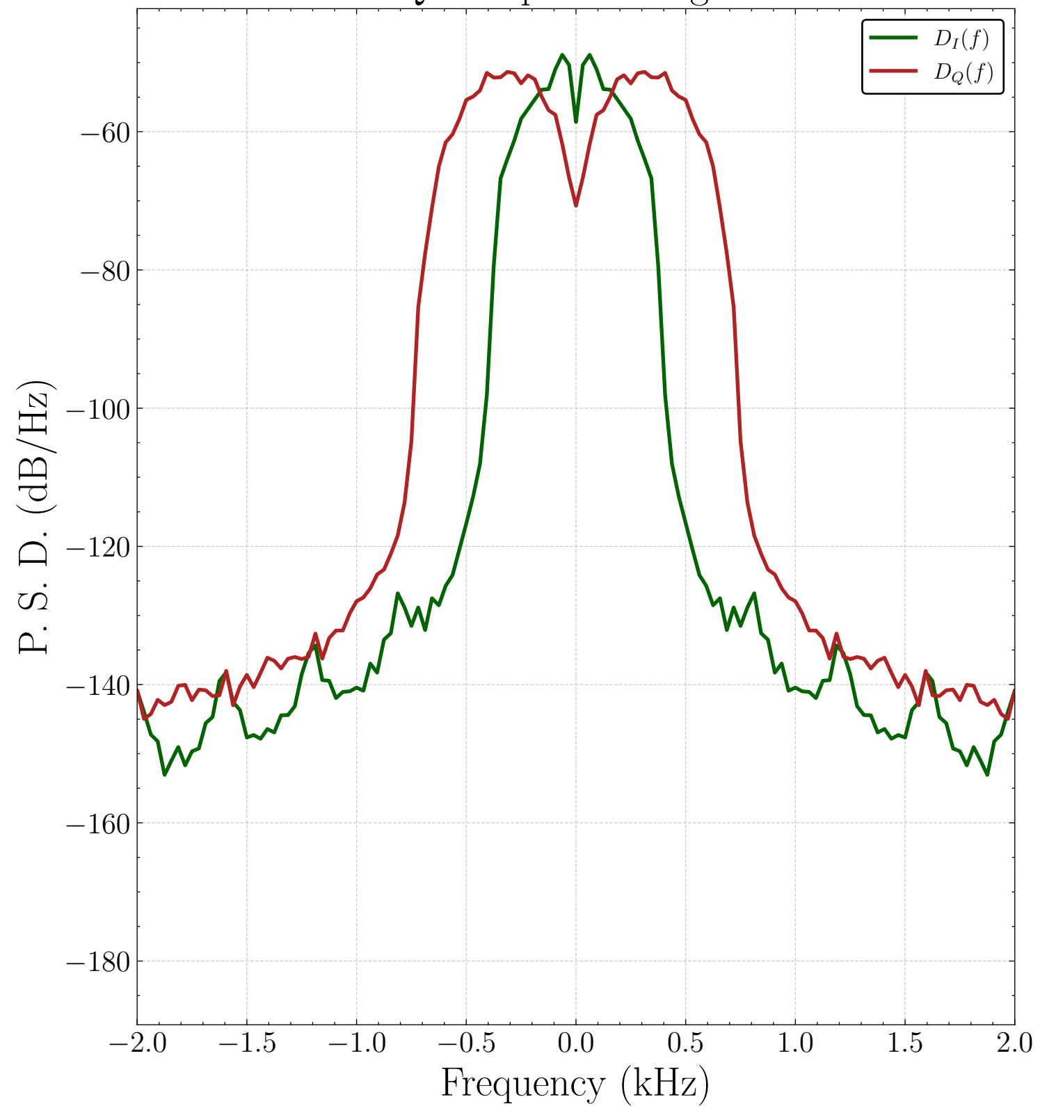
IQ Components Signals
