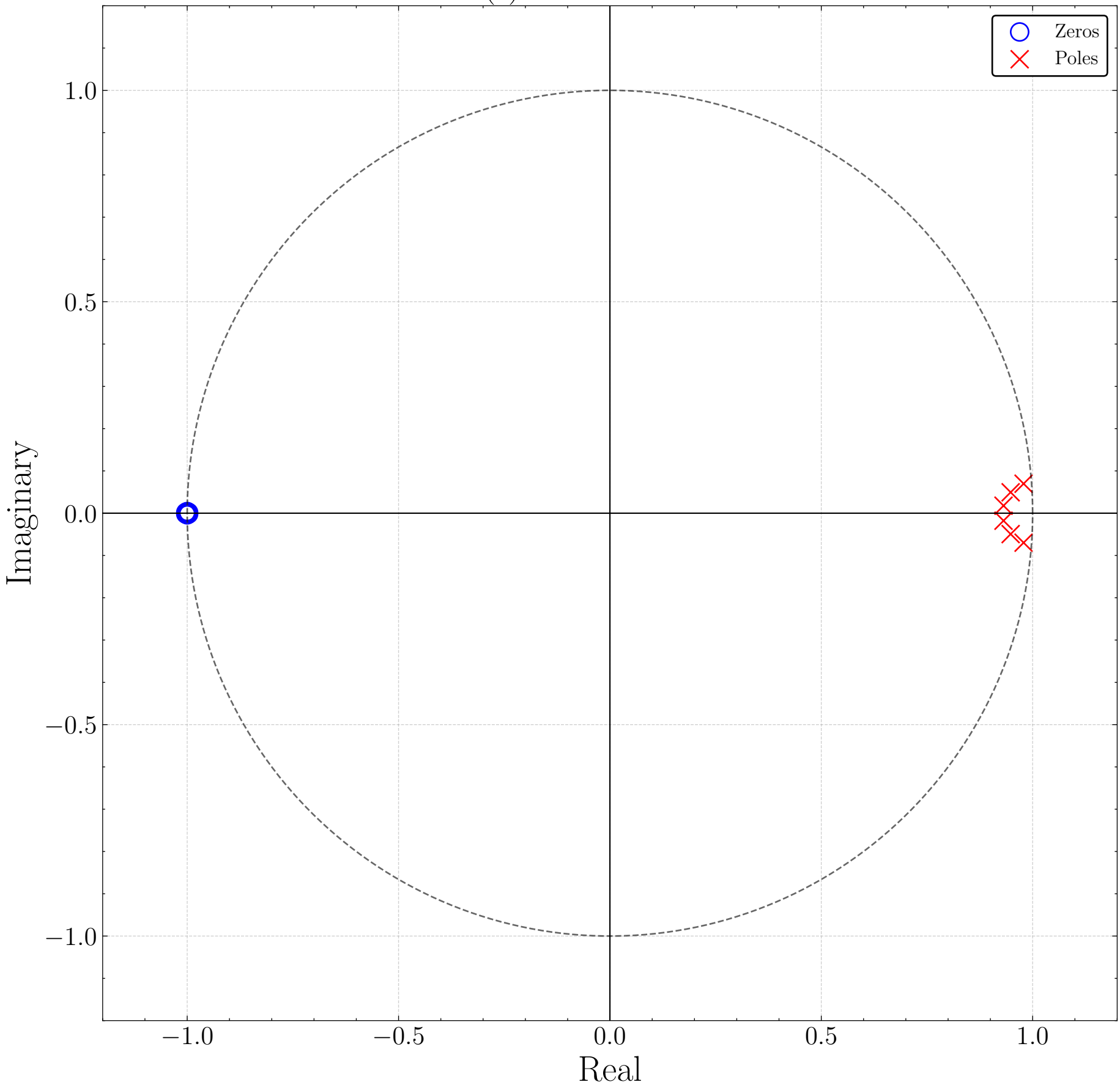
h(t) Poles and Zeros
