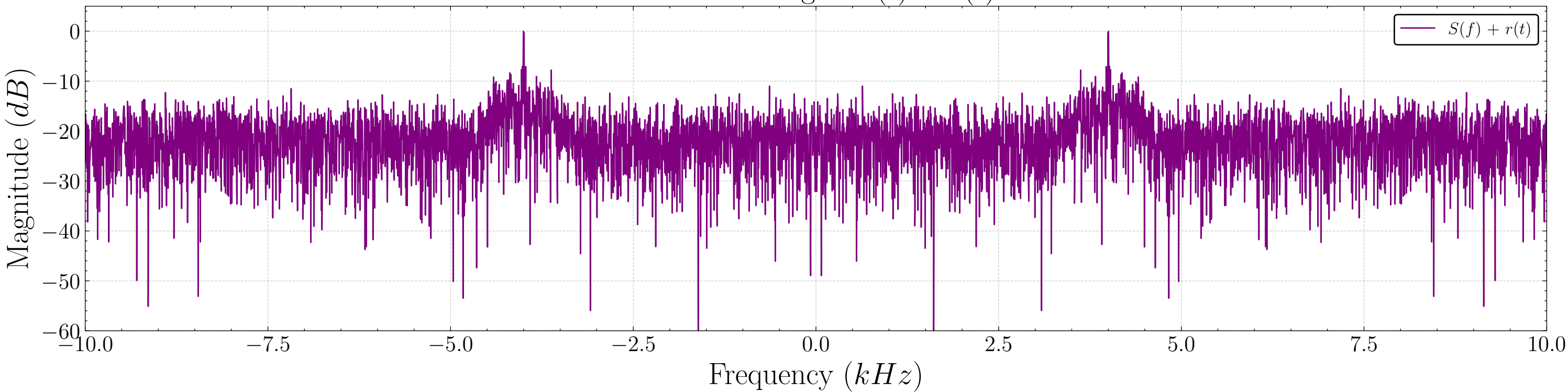
Modulated Signal s(t) + r(t)
