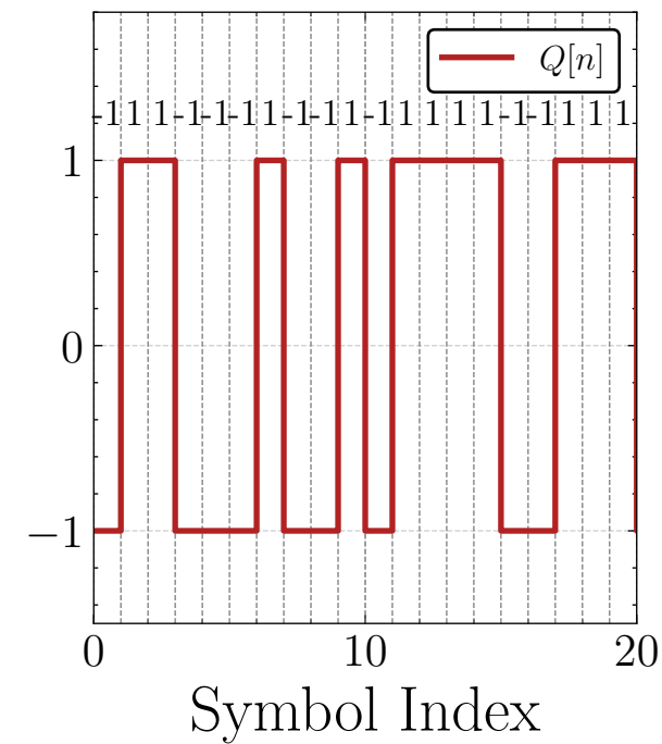
With Rect Pulse Modulation
