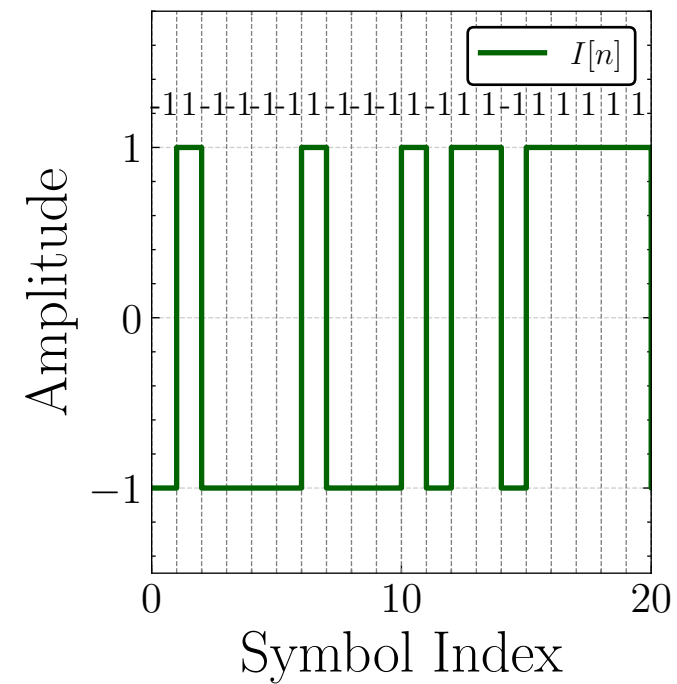
With Rect Pulse Modulation
