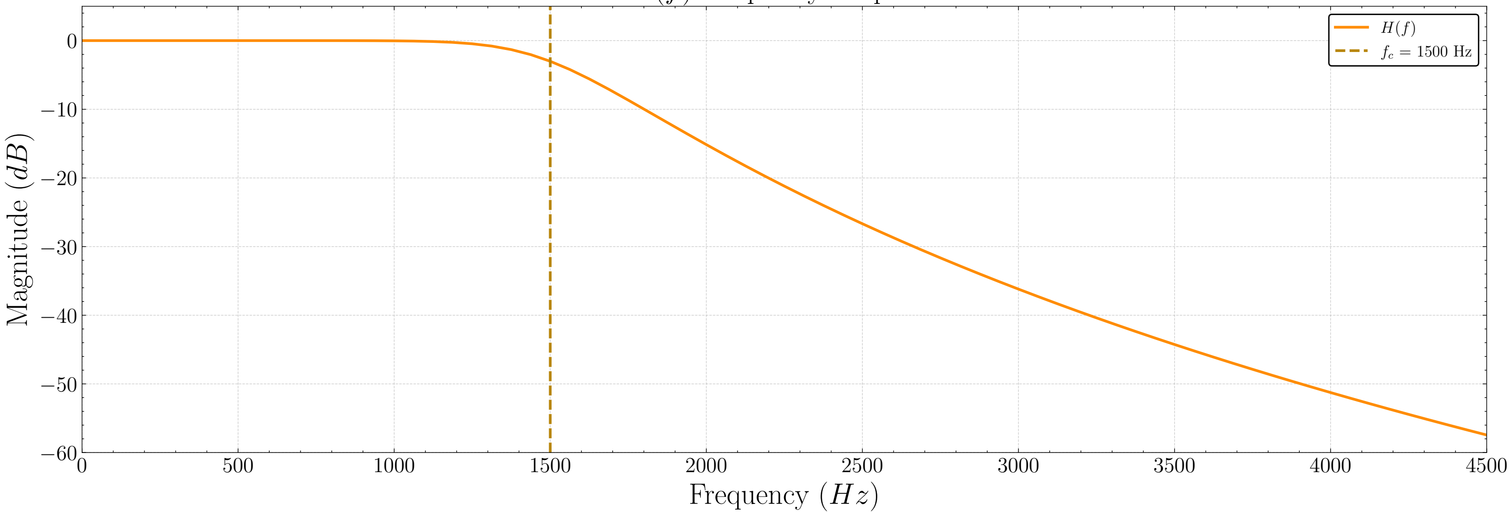
H(f) Frequency Response
