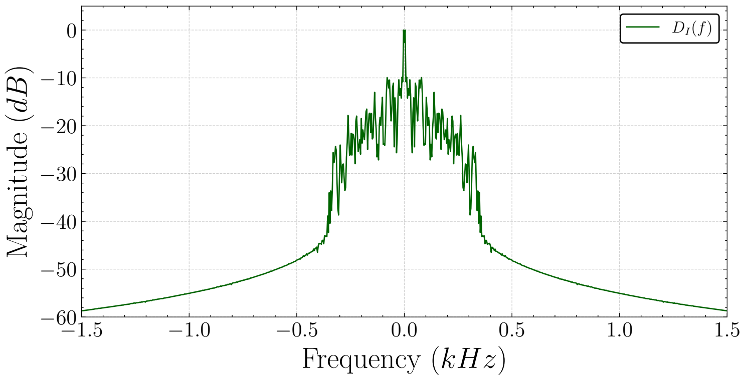
I Channel Stream
