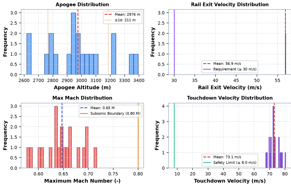
Monte Carlo Output Distributions & Requirement Compliance
