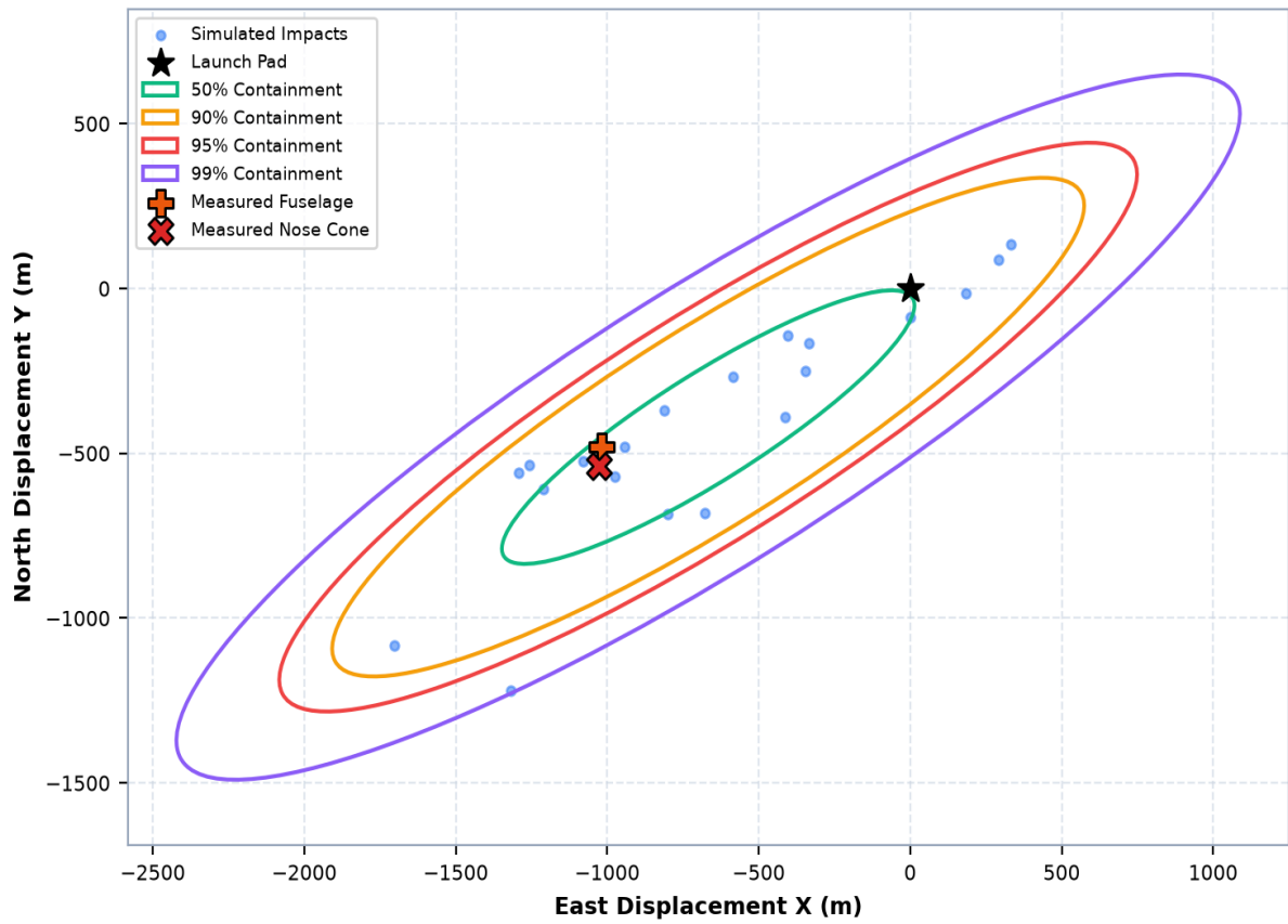
Monte Carlo 2D Ground Dispersion & Containment Ellipses (20 Cases)
