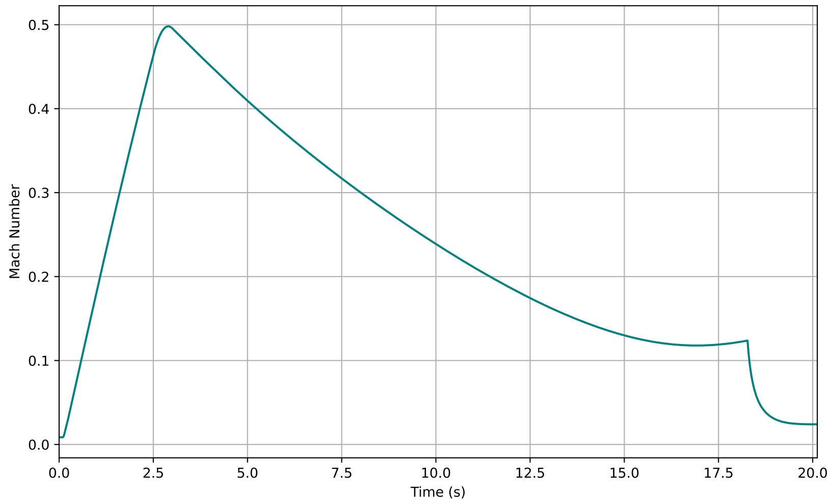
Mach Number vs Time
