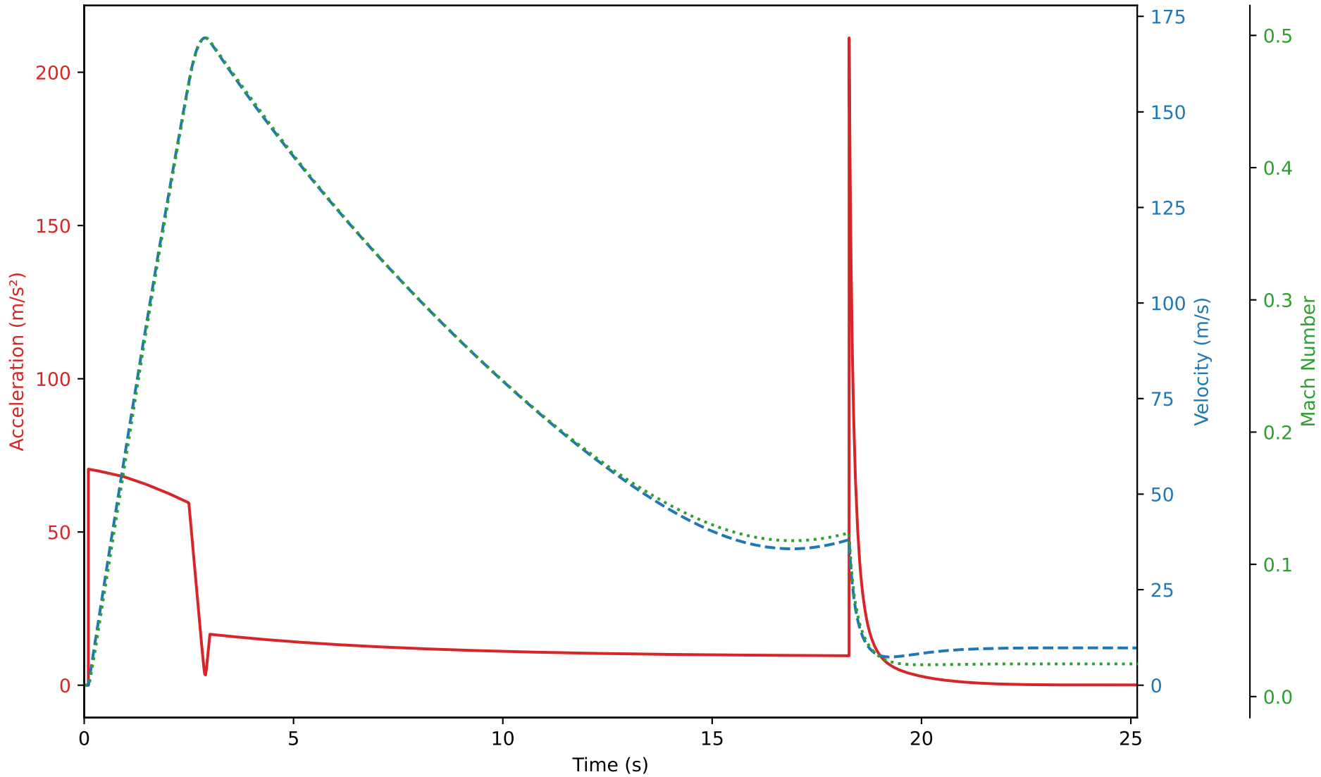
Acceleration, velocity &amp; Mach vs time
