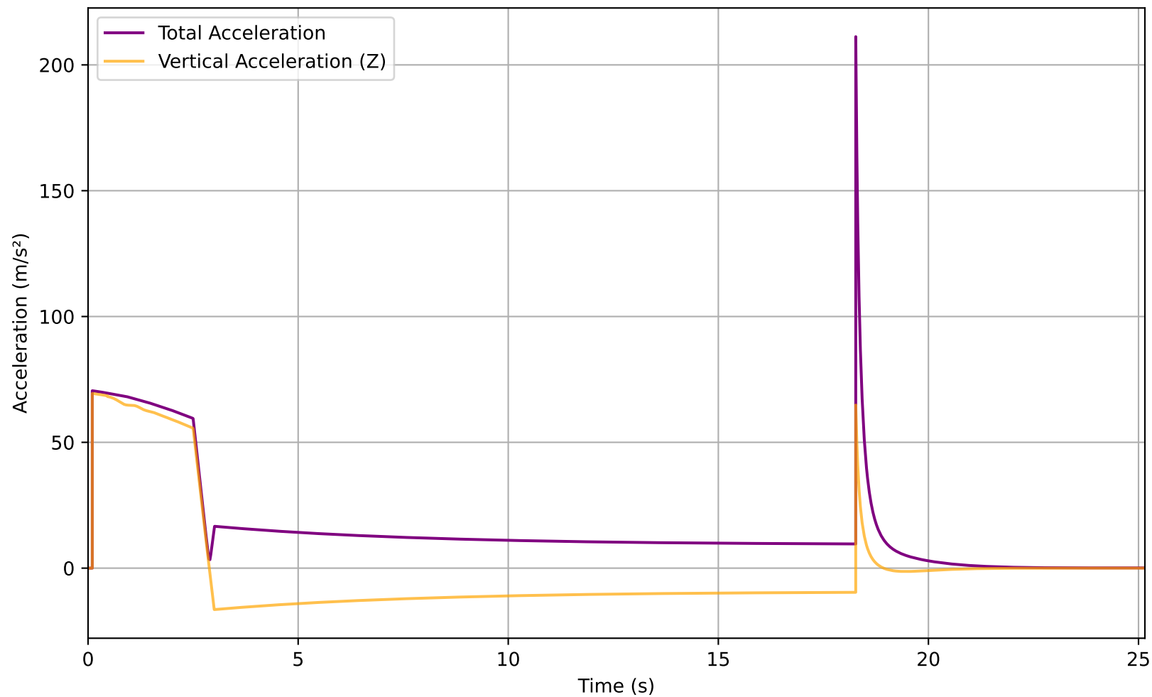
Acceleration vs Time
