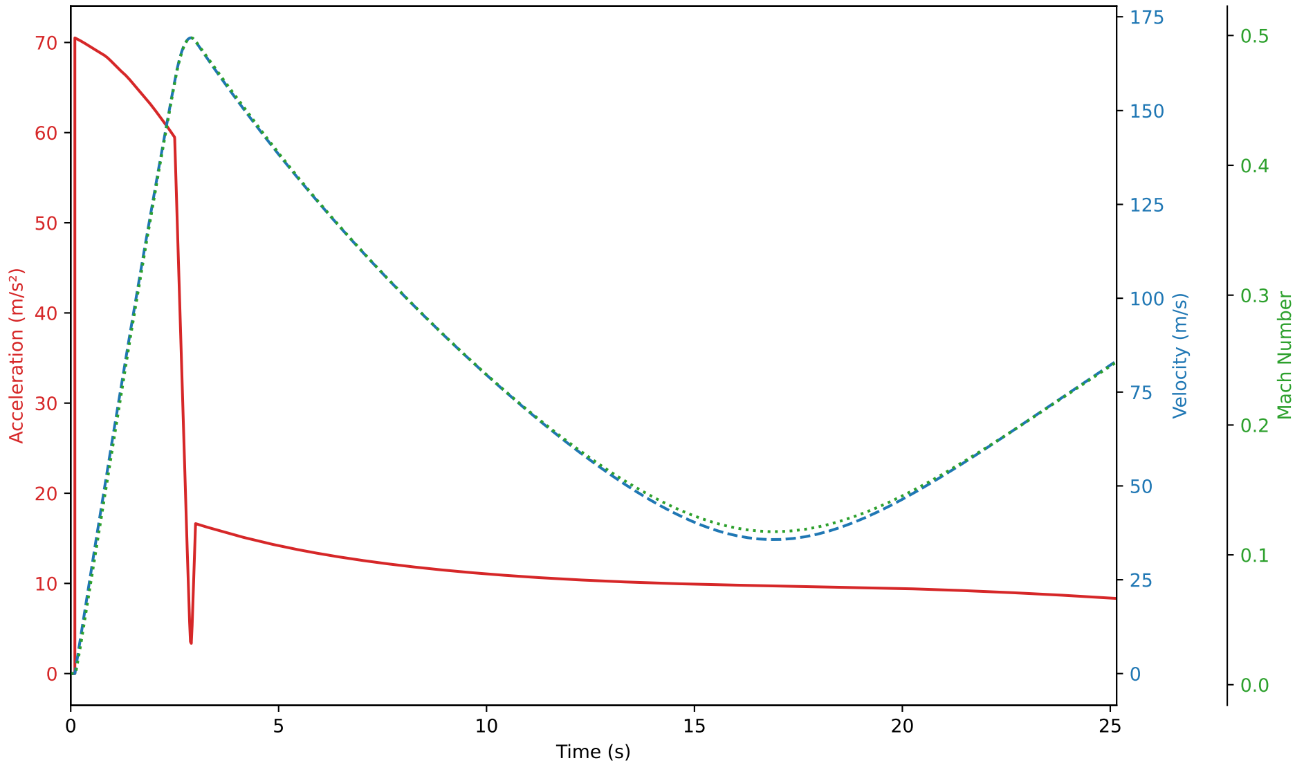
Acceleration, Velocity & Mach vs Time
