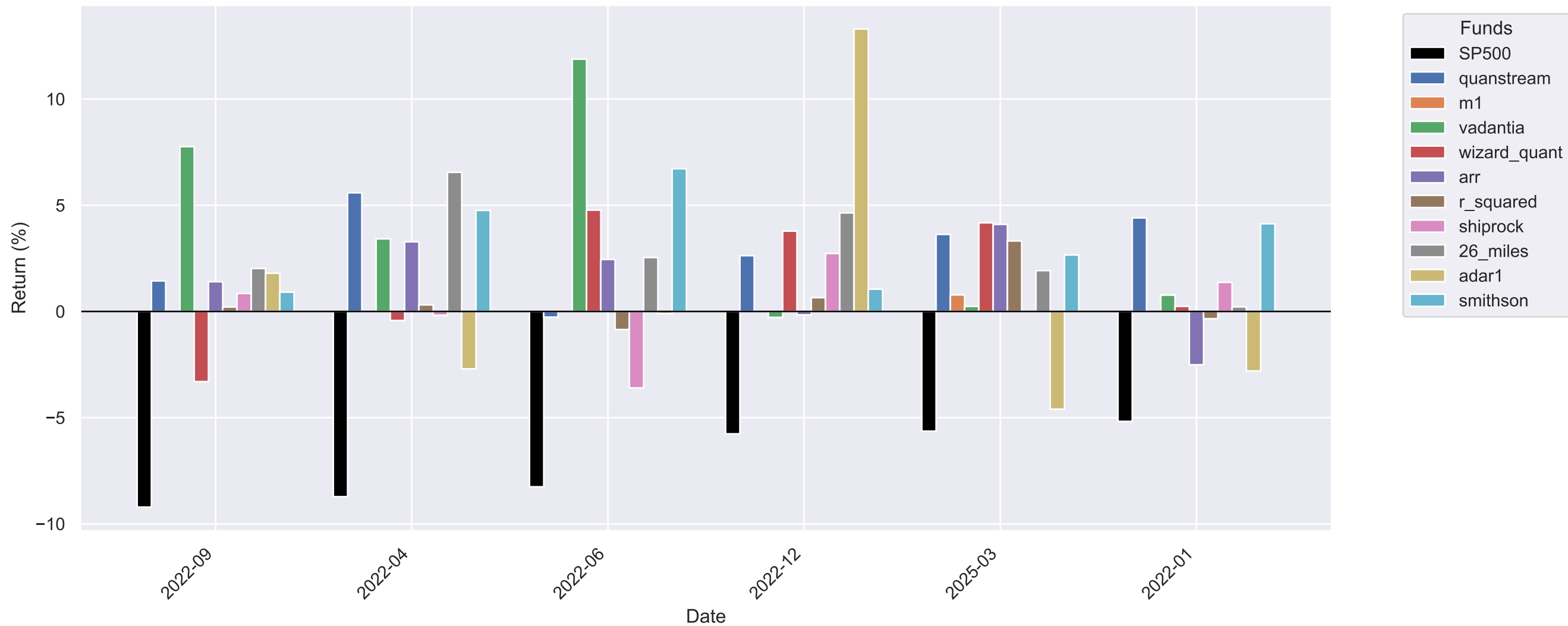
Performance During Worst 10% SP500 Months (Since 2022, Selected Funds)
