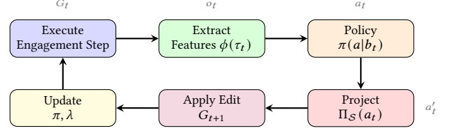
Figure 2: The SAGE adaptation loop. At each step, the system executes an engagement step with the current architecture G_t , extracts trace features, queries the policy for an edit action, projects the action to satisfy hard constraints, applies the edit to obtain G_{t+1} , and updates the policy and Lagrange multiplier based on observed utility, cost, and risk signals.
