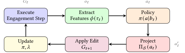
Figure 2: The SAGE adaptation loop. At each step, the system executes an engagement step with the current architecture G_t , extracts trace features, queries the policy for an edit action, projects the action to satisfy hard constraints, applies the edit to obtain G_{t+1} , and updates the policy and Lagrange multiplier based on observed utility, cost, and risk signals.
