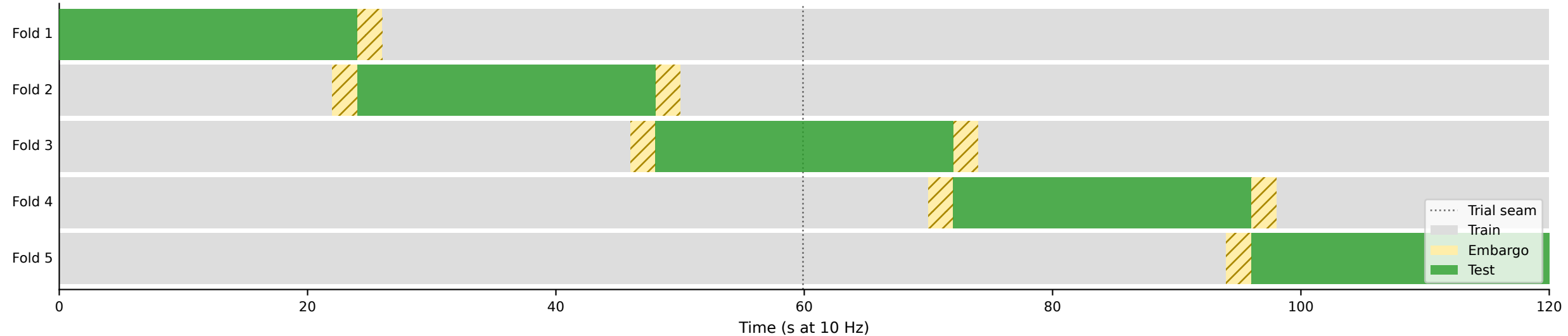
fig06 — Cross-validation structure | RH (5-fold contiguous | embargo = 20 samples = 2.0 s [implemented])
