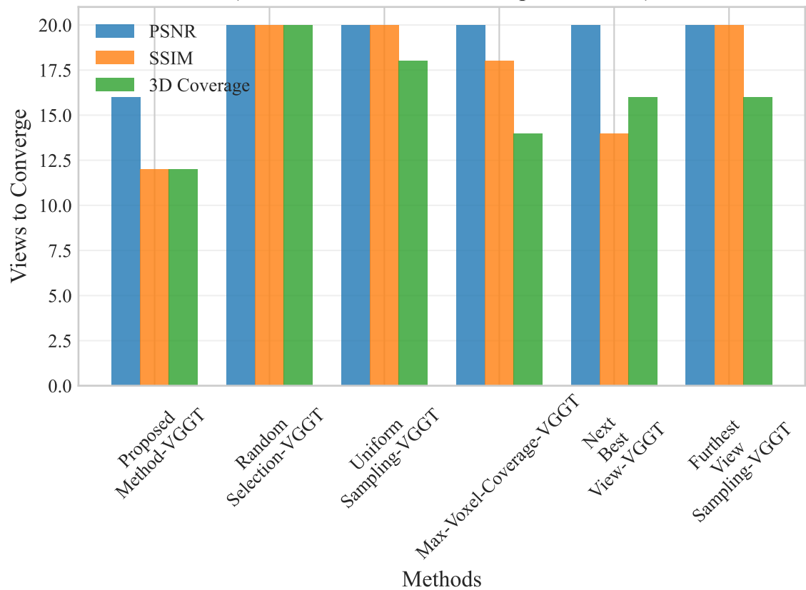
(b) Convergence Speed Analysis (Views to reach 95% of max performance)
