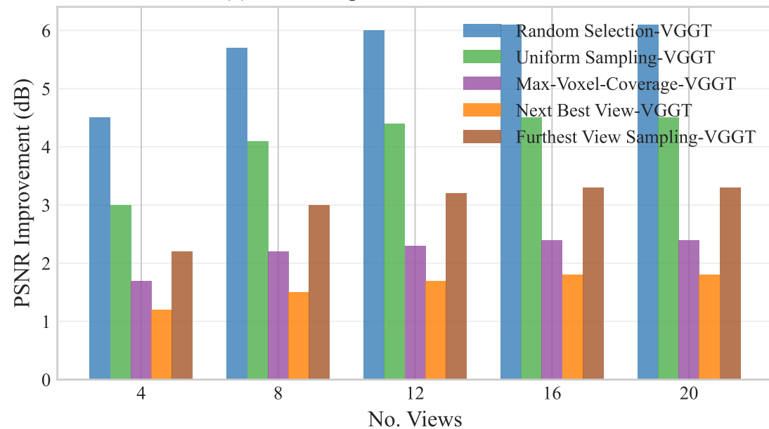
(a) PSNR Improvement Over Baselines
