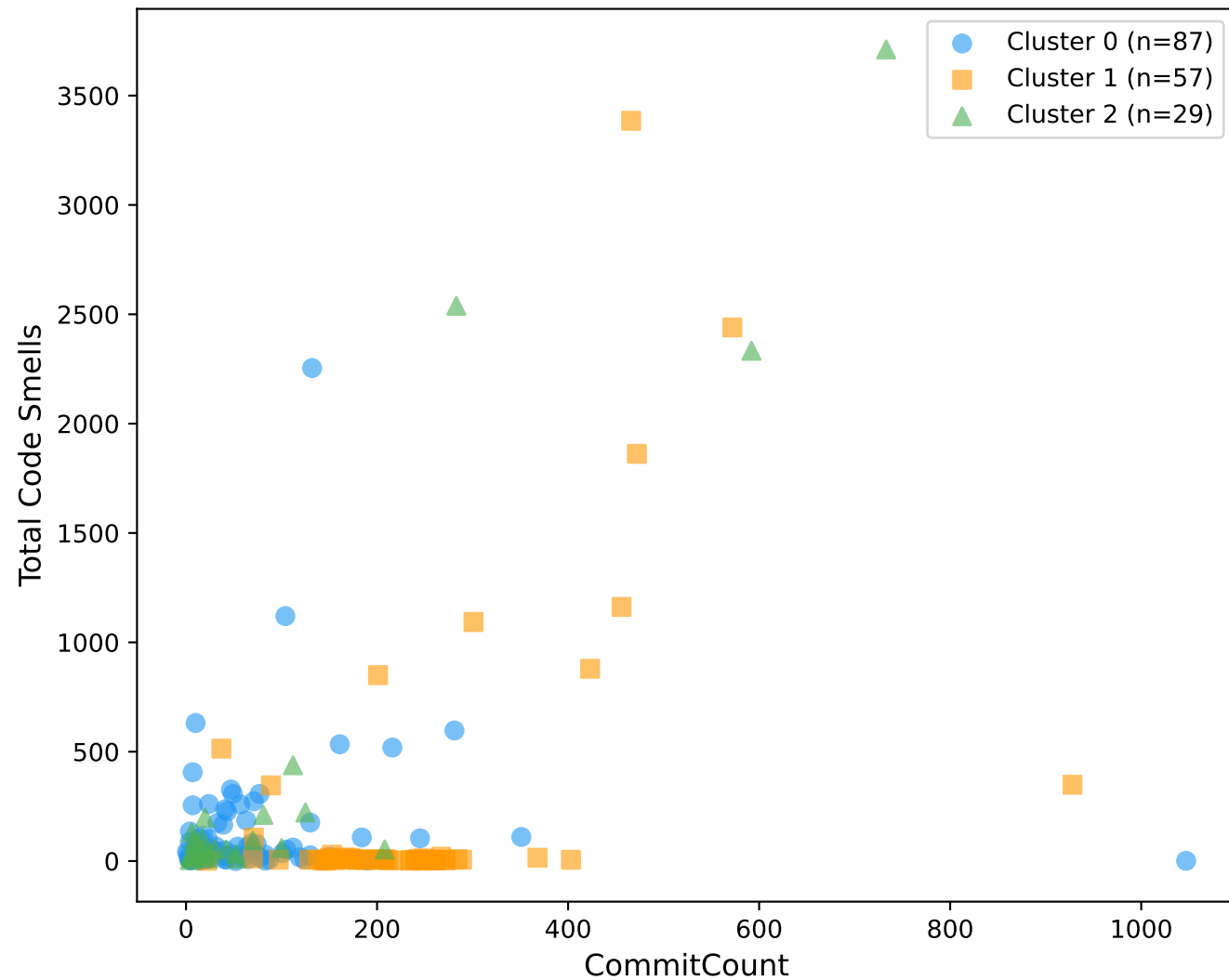
(a) Code Smells vs. Commits
