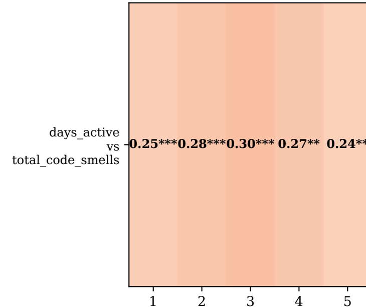
Days Active vs Total Code Smells
