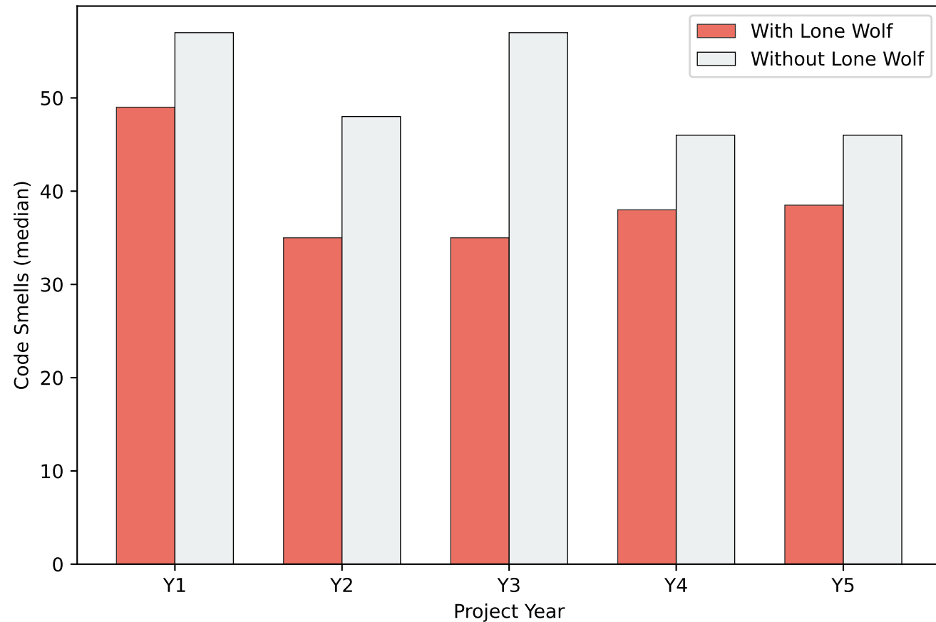
Code Smells × Lone Wolf
