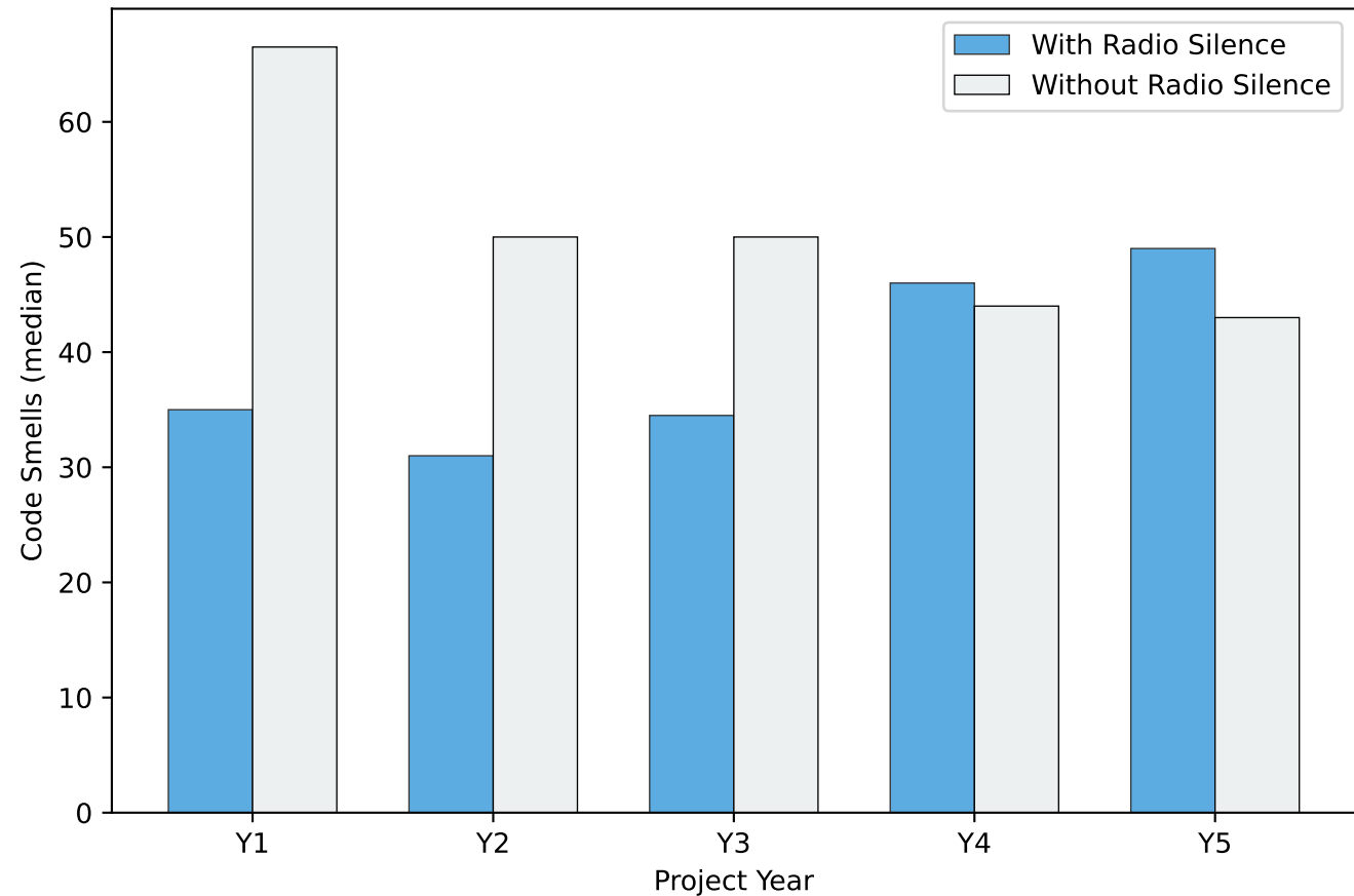
Code Smells × Radio Silence
