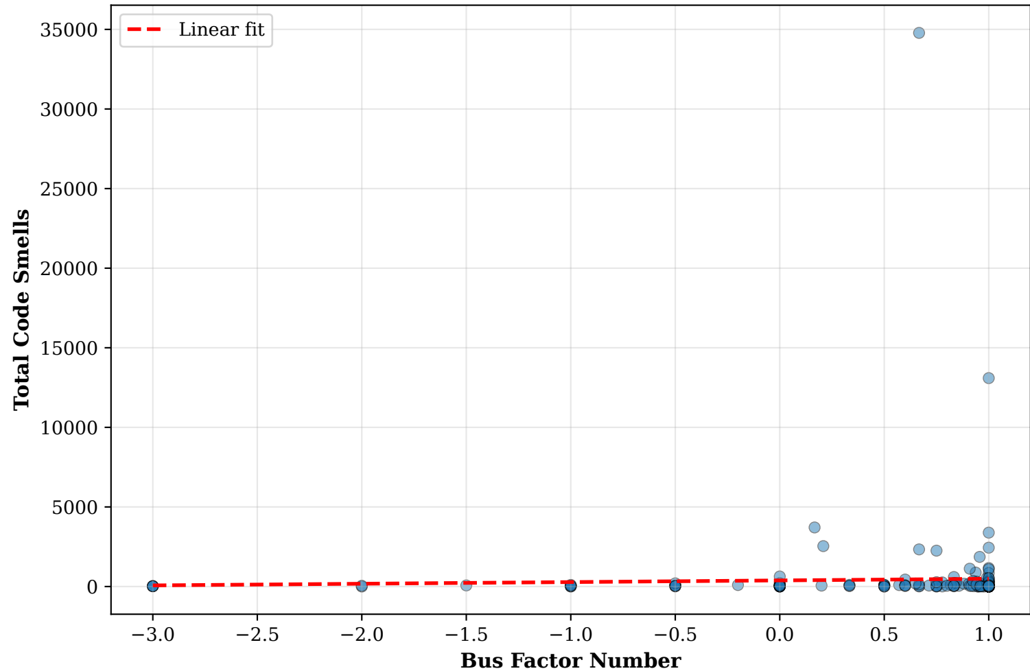
Bus Factor vs Code Smells (rho=-0.254, p=0.0004)
