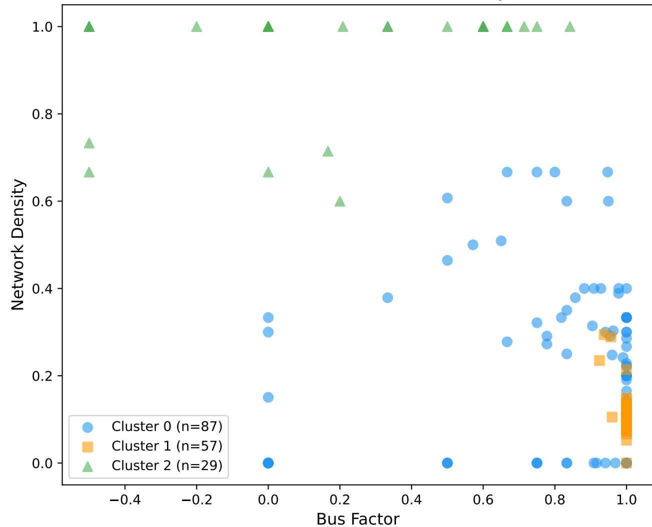
(b) Bus Factor vs. Network Density
