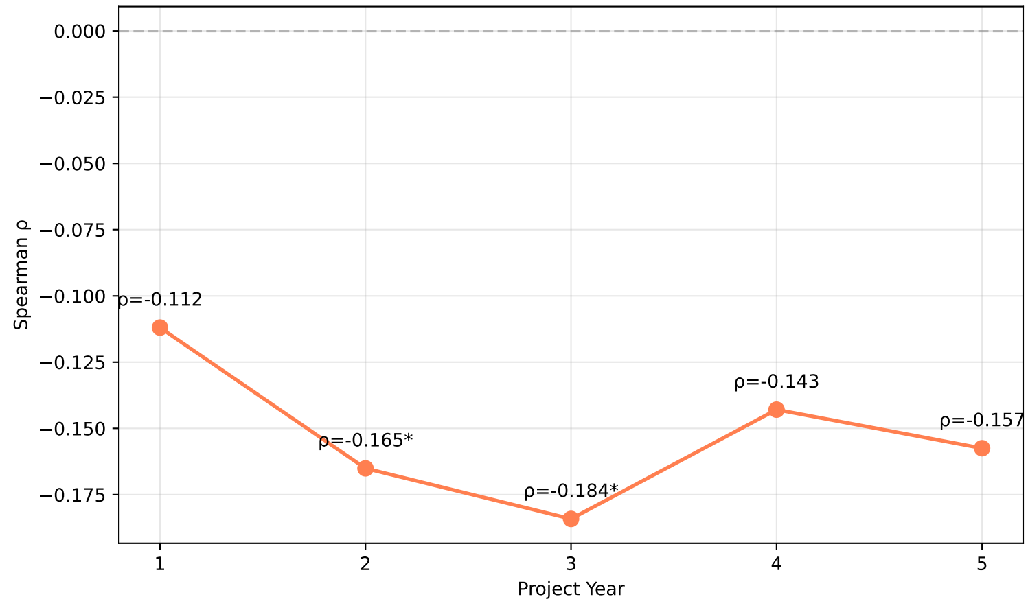
Evolution: Bus Factor \times Code Smells Correlation
