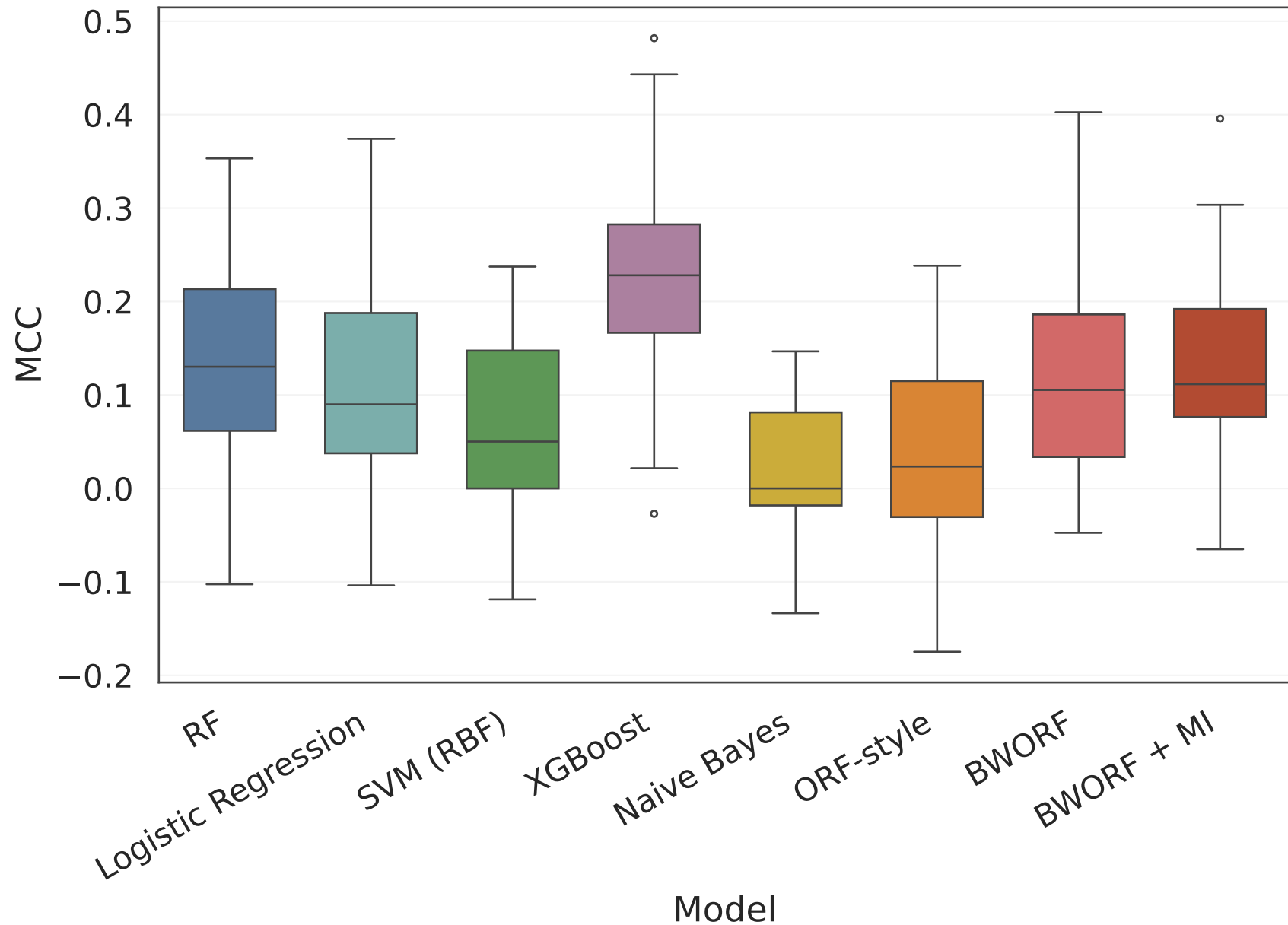
Multiclass DILI Benchmark: MCC Distributions
