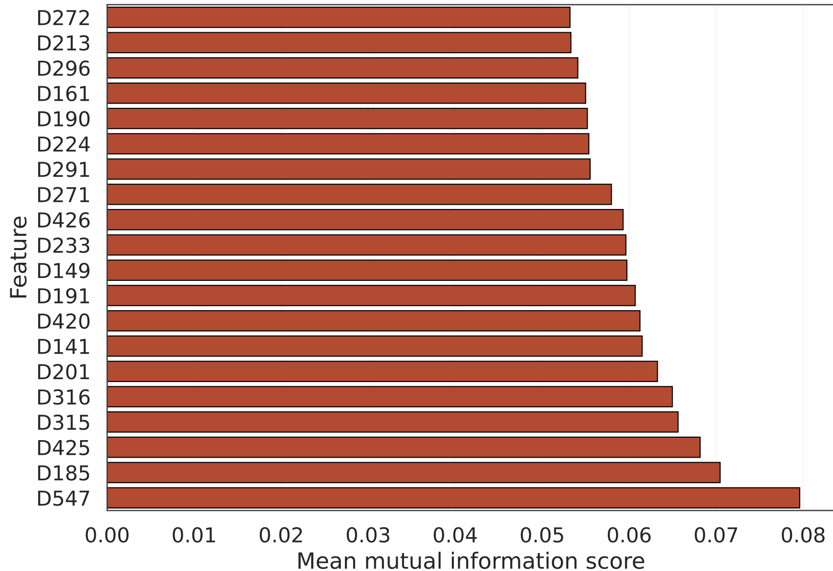
Top 20 MI-Ranked Features for BWORF + MI
