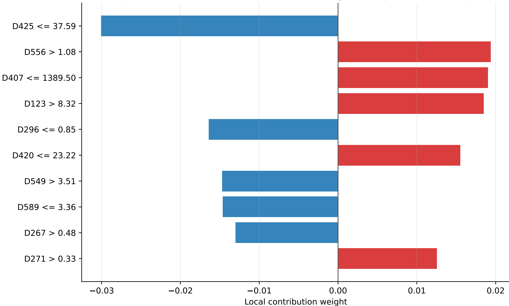
High-confidence correct: sample 79 (ID 3763) | true=High, explained=High
