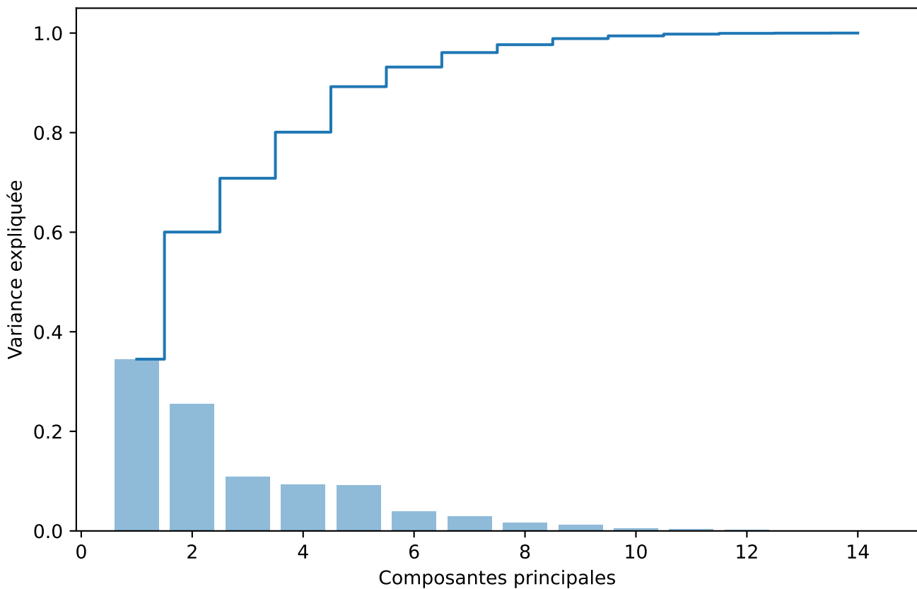
Scree Plot
