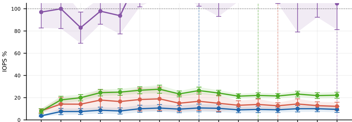
IOPS utilization
