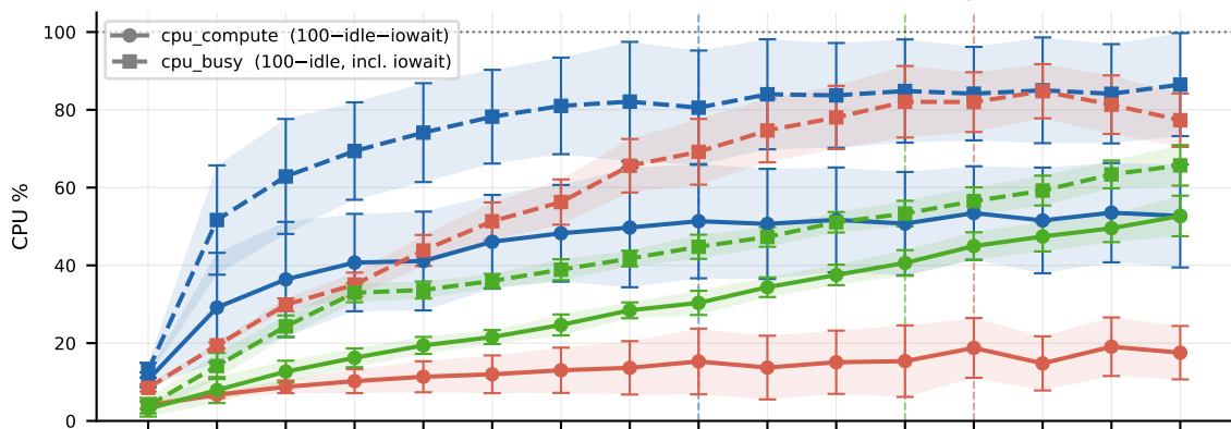
CPU utilization (solid = compute, dashed = busy)
