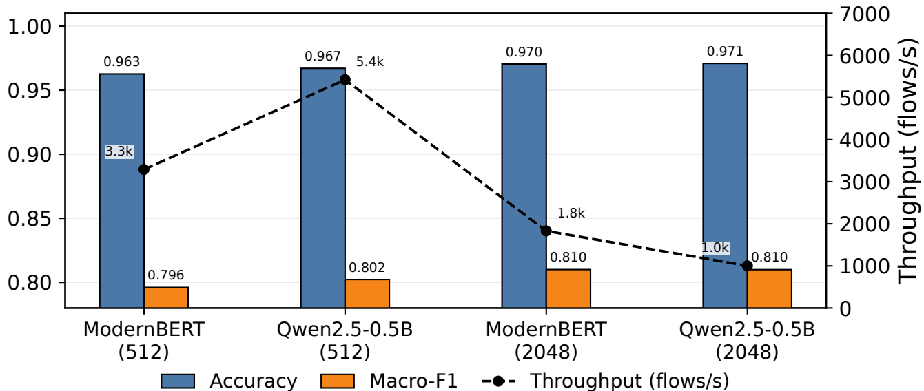
Detection Score
