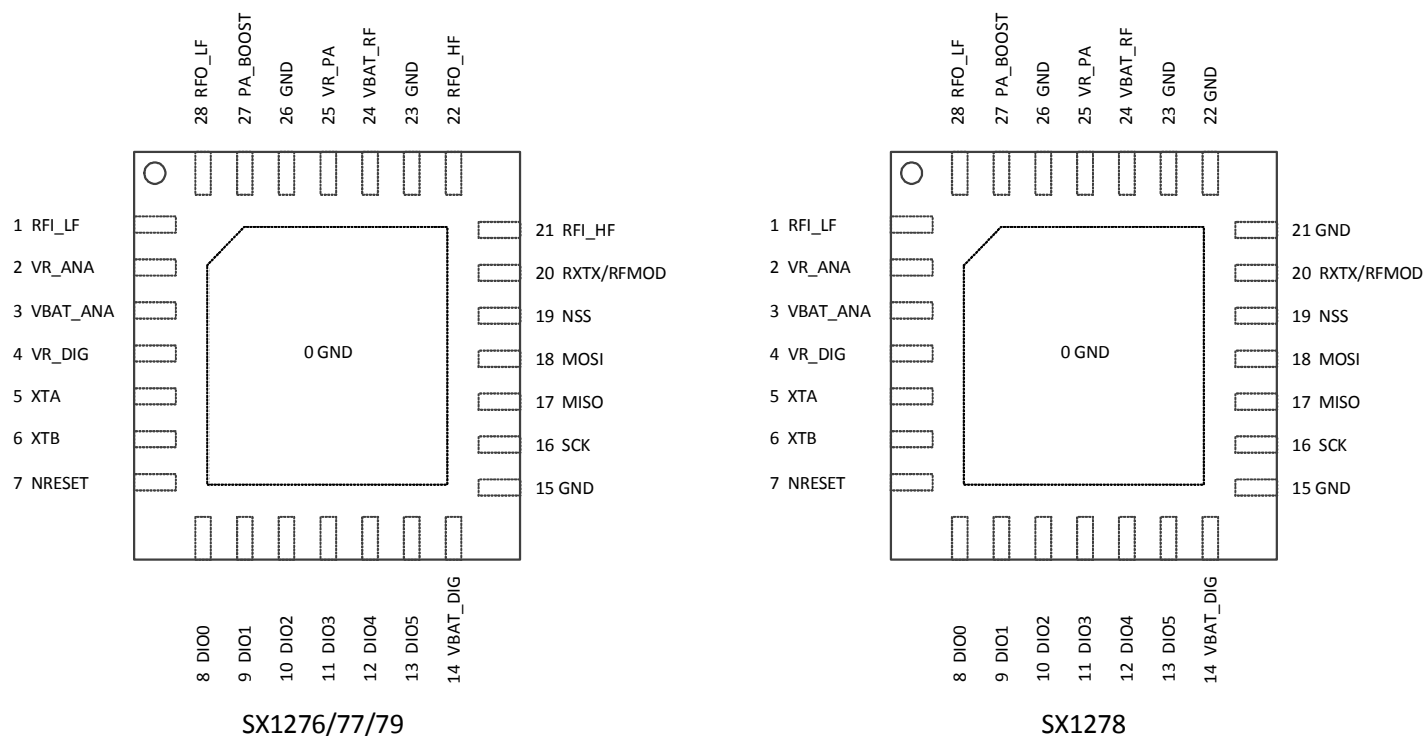
Figure 2. Pin Diagrams
