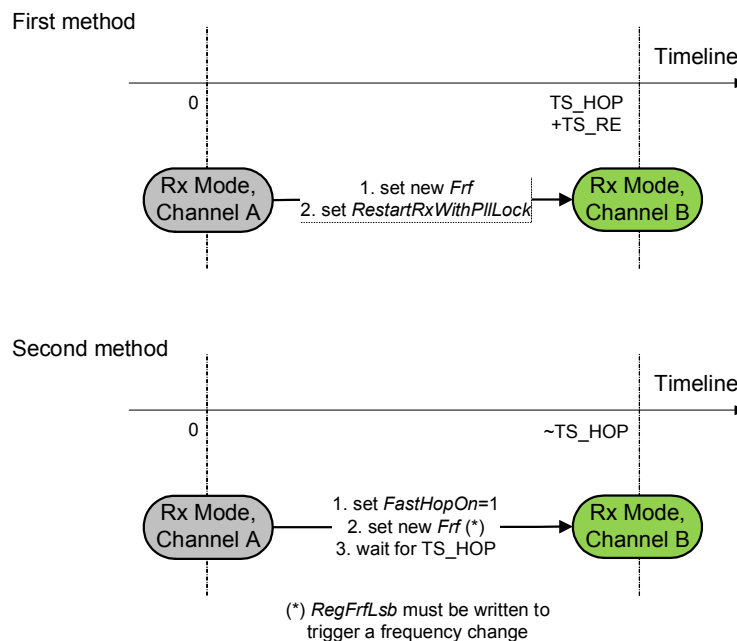
Figure 21. Receiver Hopping
