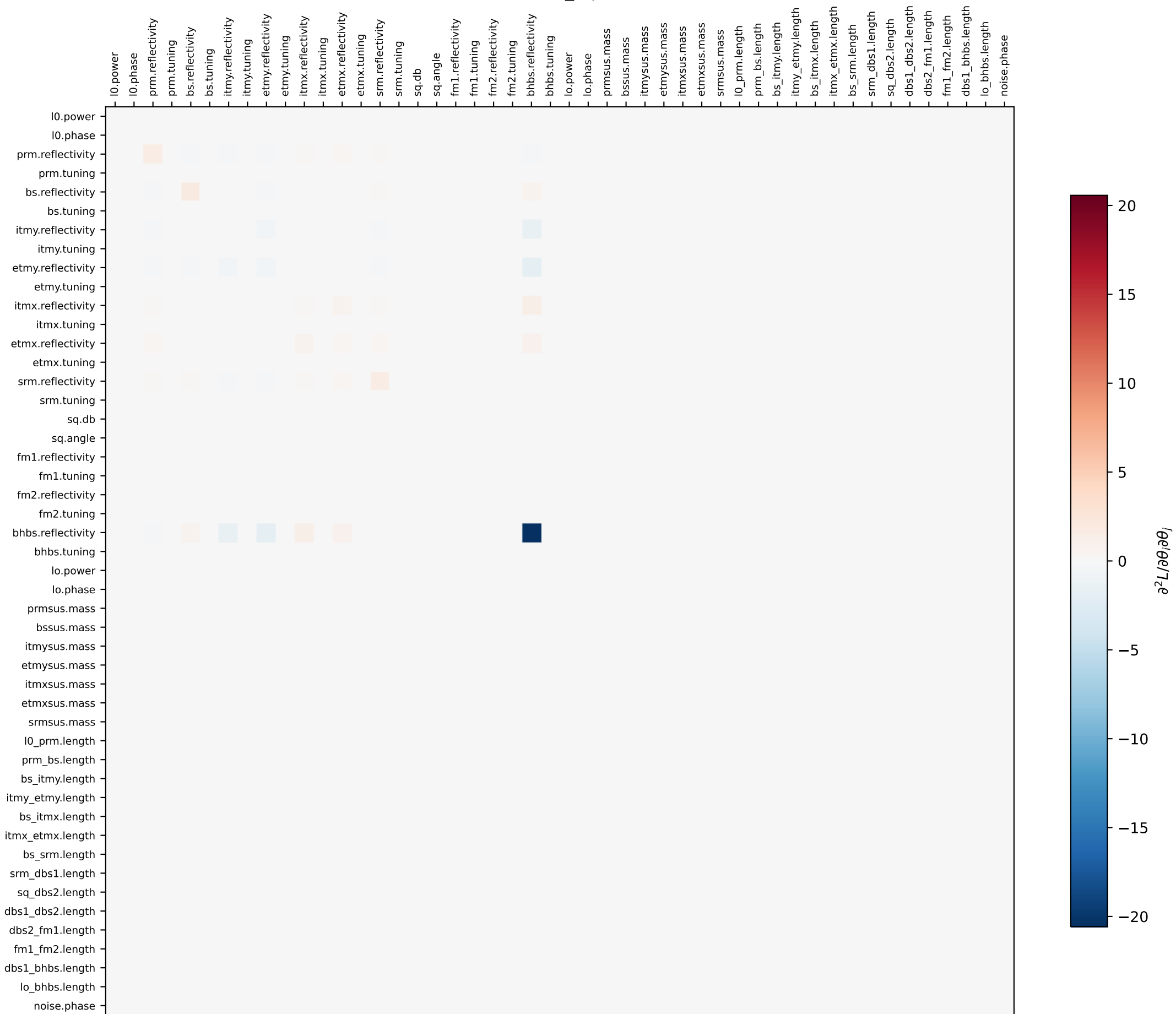
Hessian (at rand_0 parameters)
