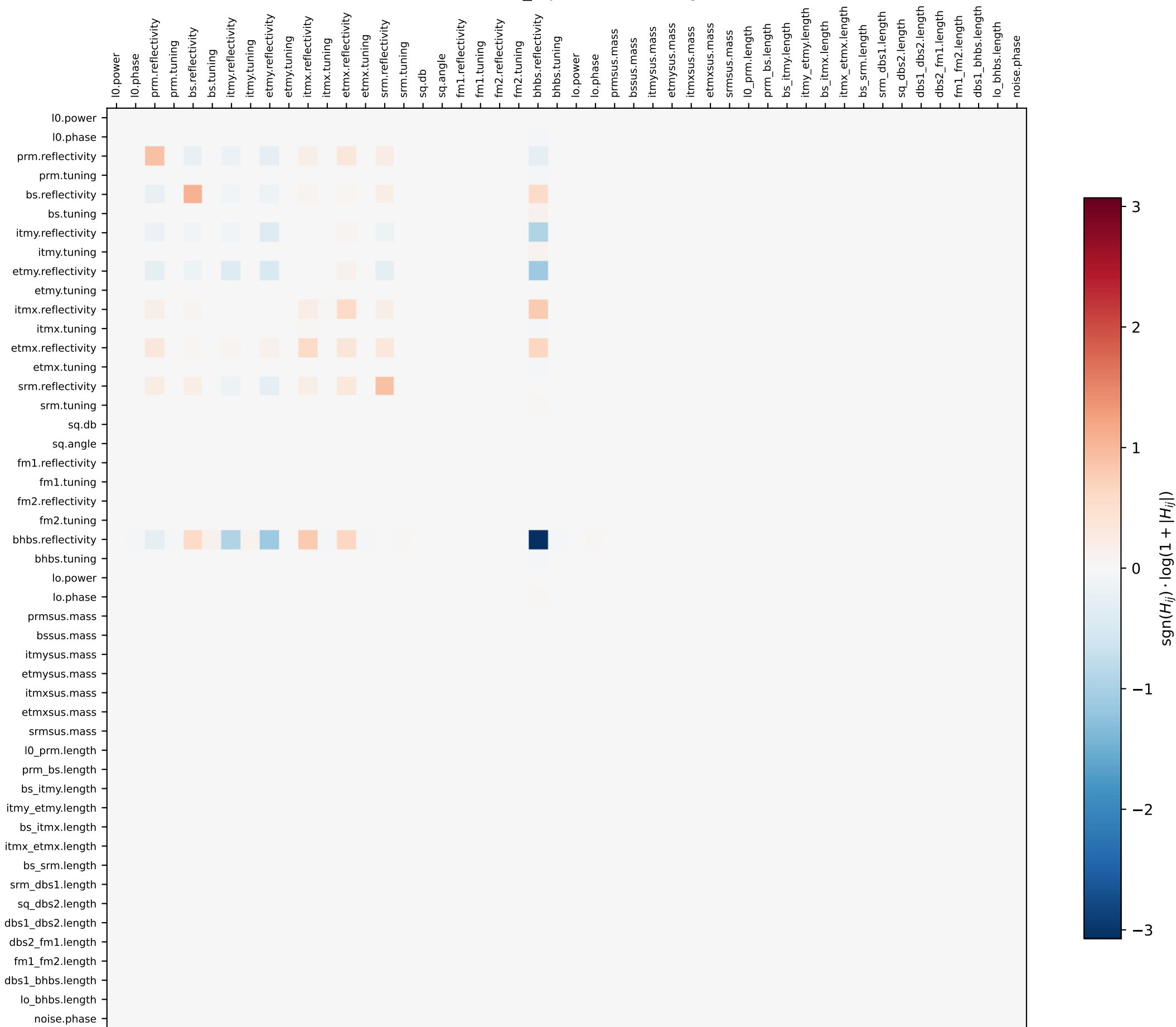
Hessian (at rand_0 parameters) (log scale)
