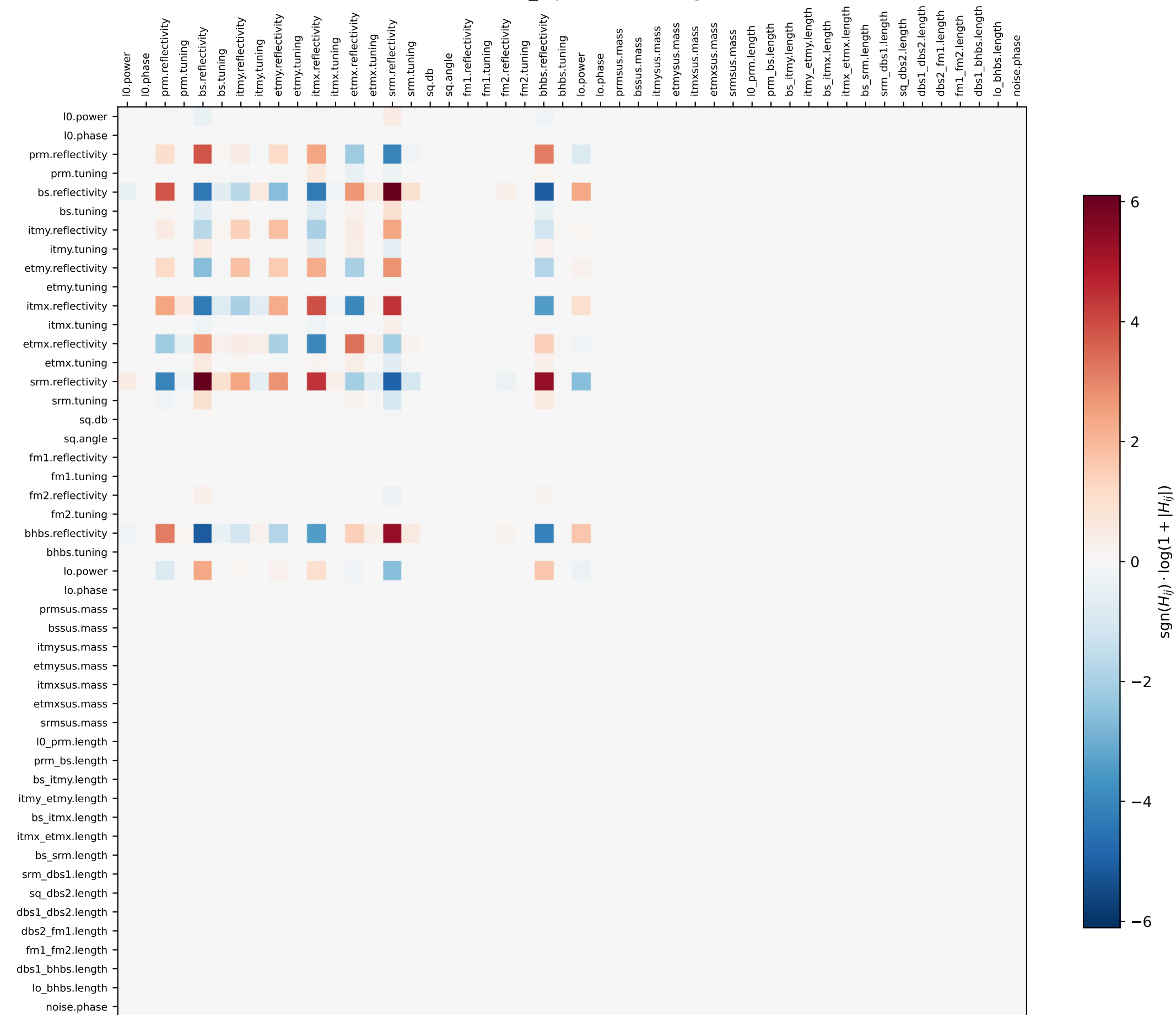
Hessian (at rand_1 parameters) (log scale)
