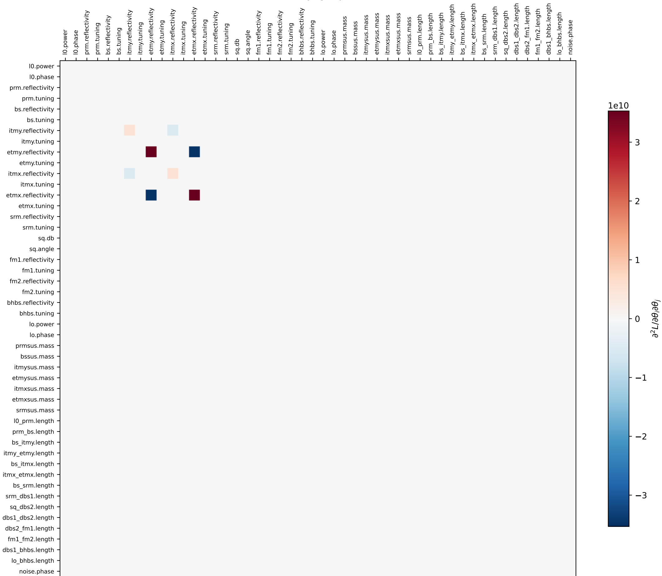
Hessian (at Voyager parameters)
