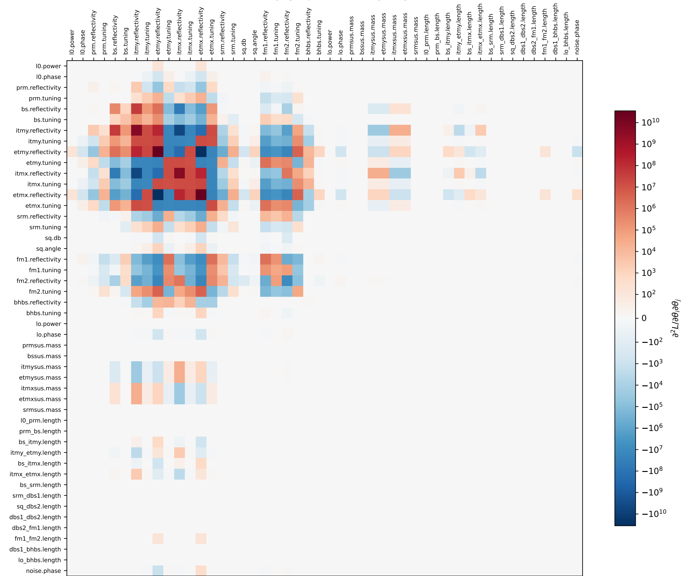
Hessian at Voyager parameters (symlog scale)
