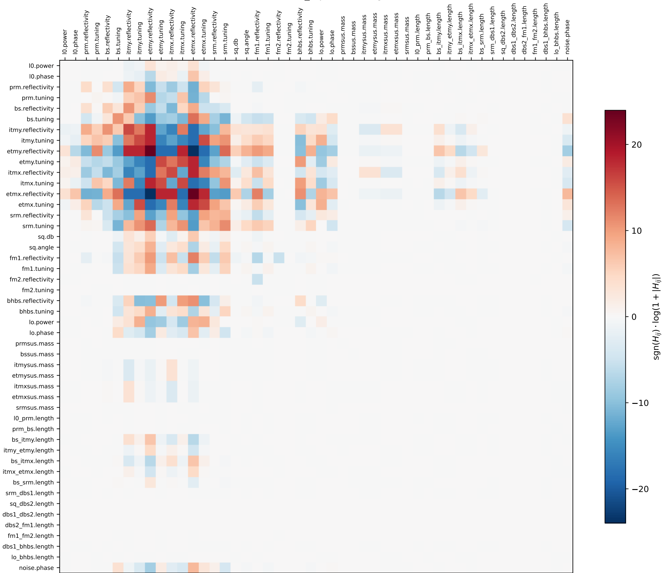
Hessian (at adam_0 params) (log scale)
