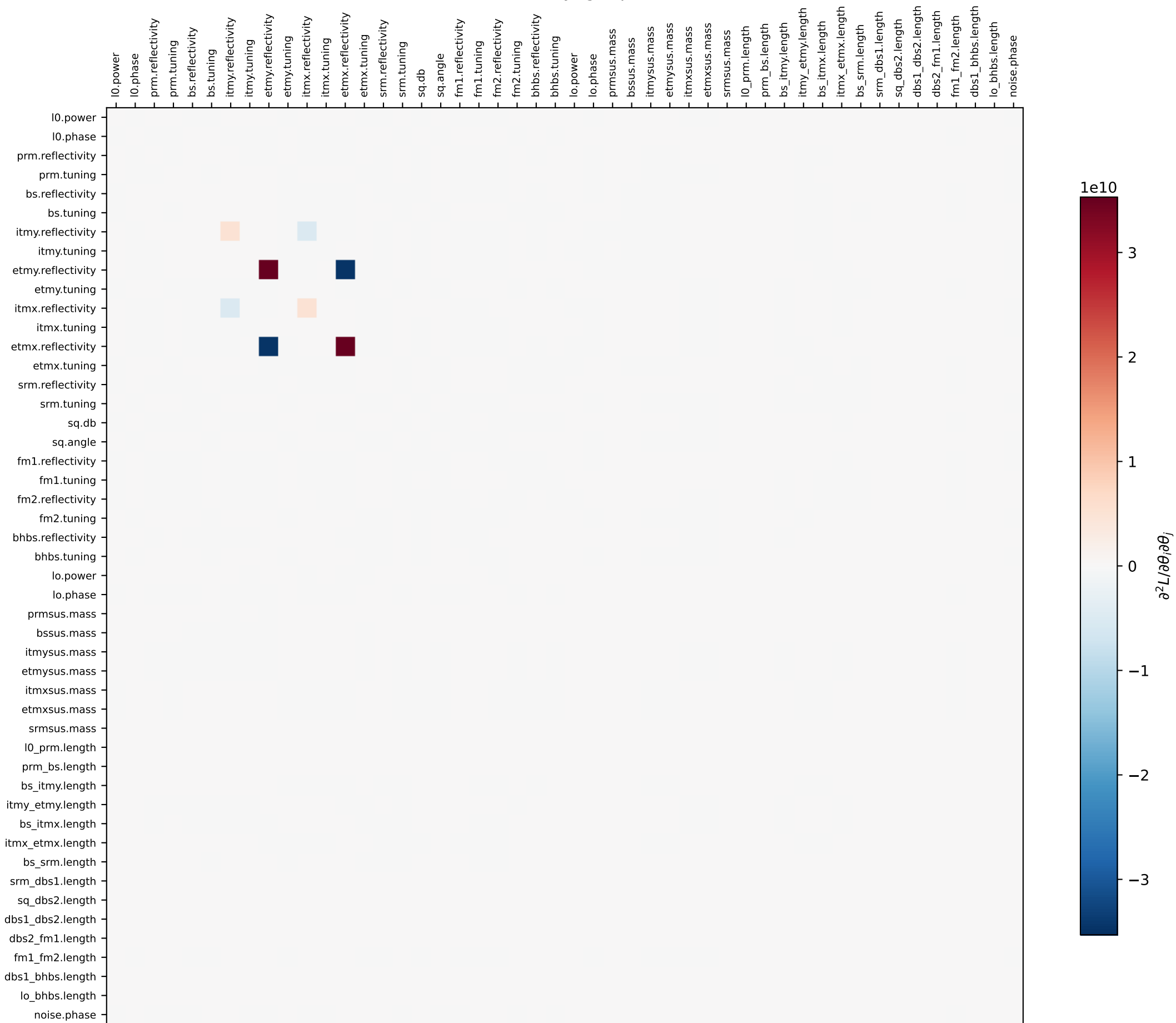
Hessian (at Voyager params)
