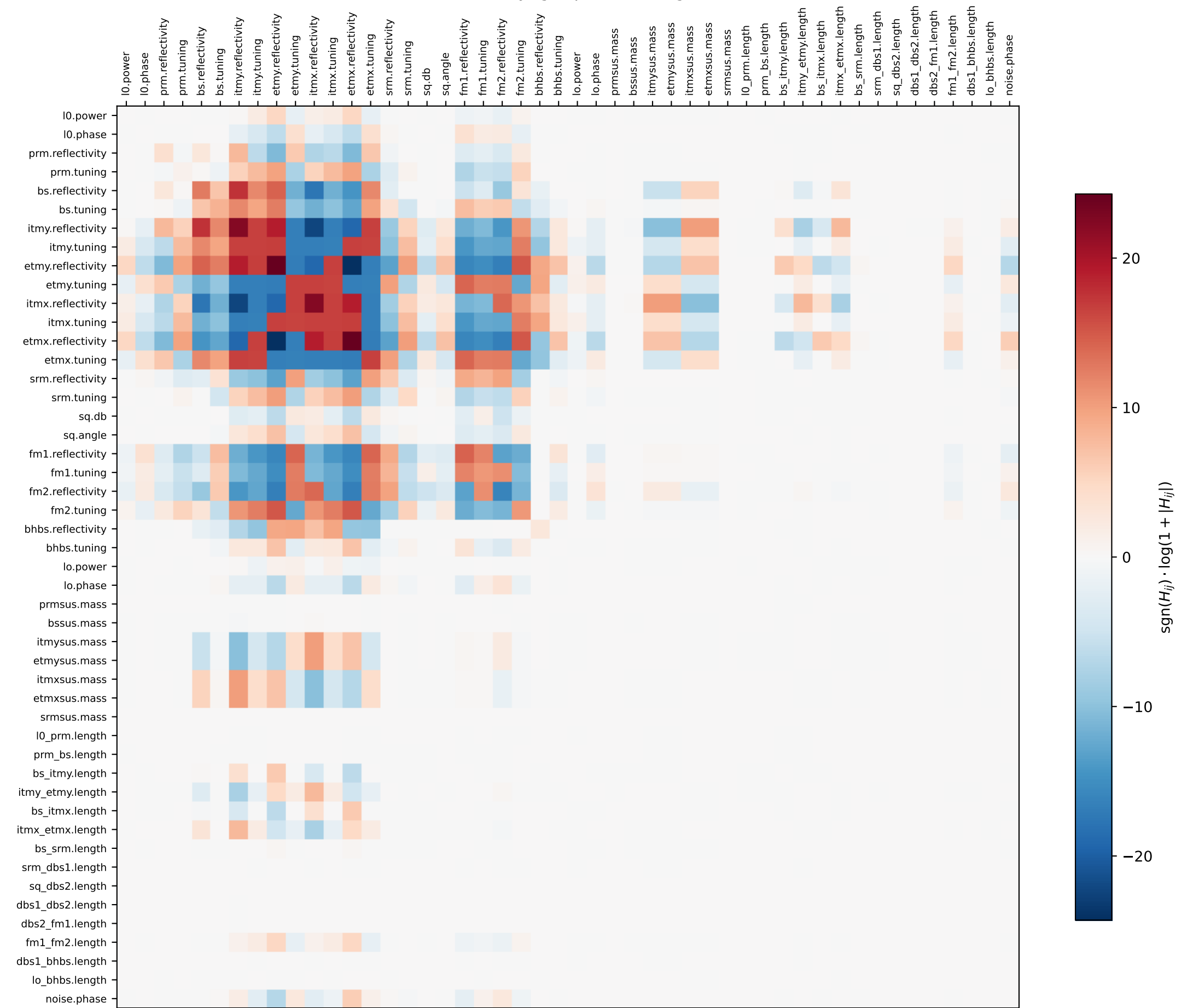
Hessian (at Voyager params) (log scale)
