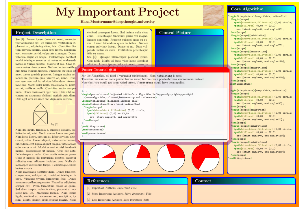
Patched tcolorbox
