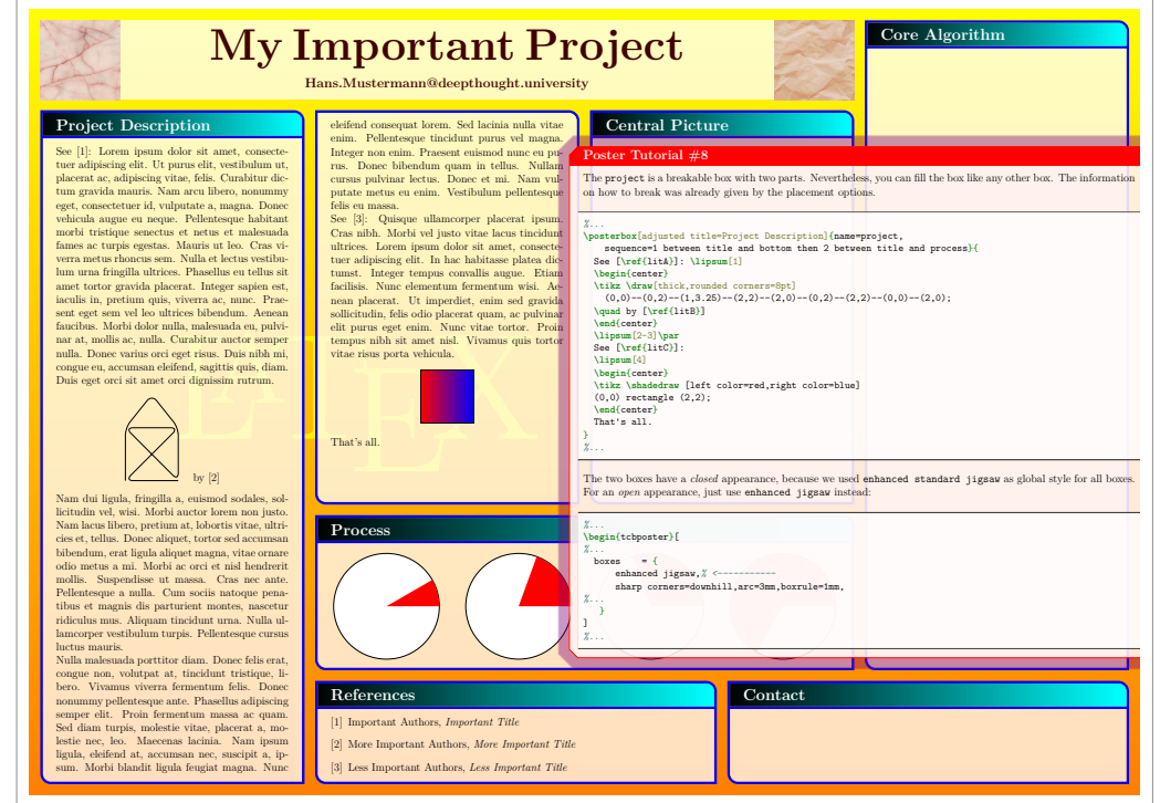
breakble-tcolorbox
