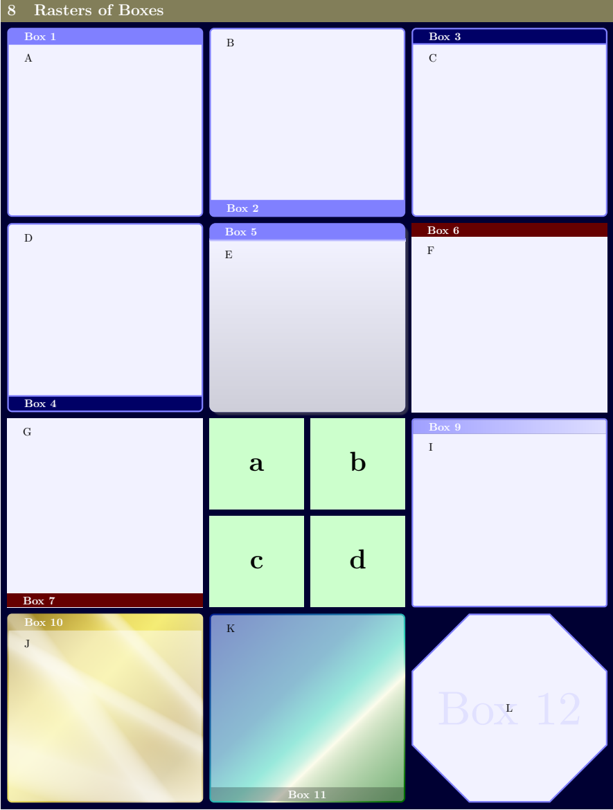
Patched tcolorbox
