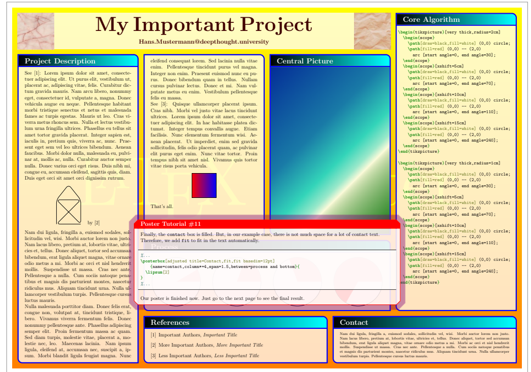
Patched tcolorbox
