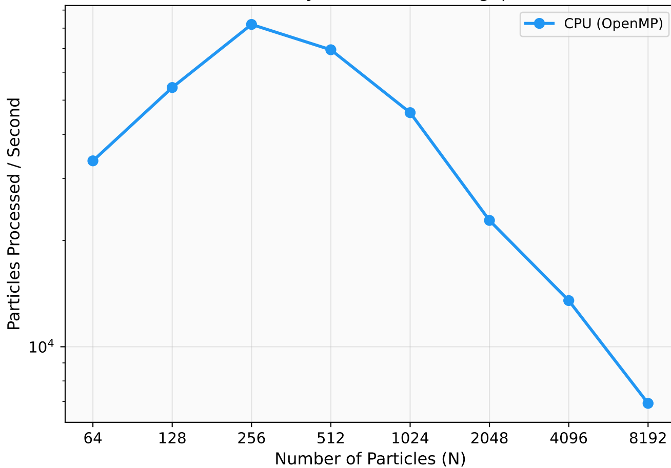
CPU N-Body: Simulation Throughput
