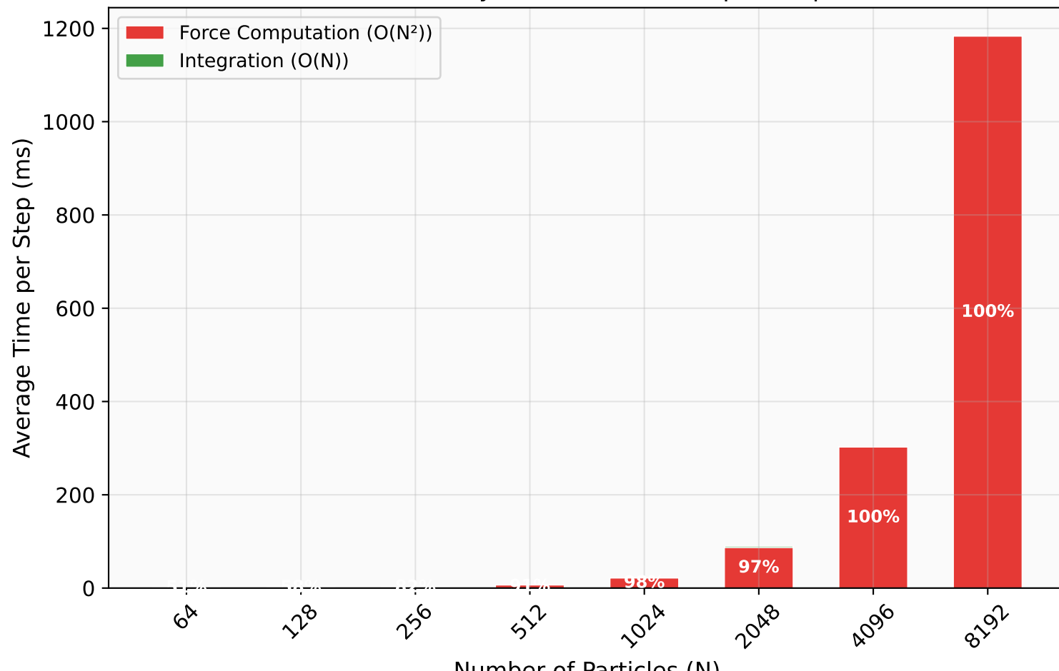
CPU N-Body: Time Breakdown per Step
