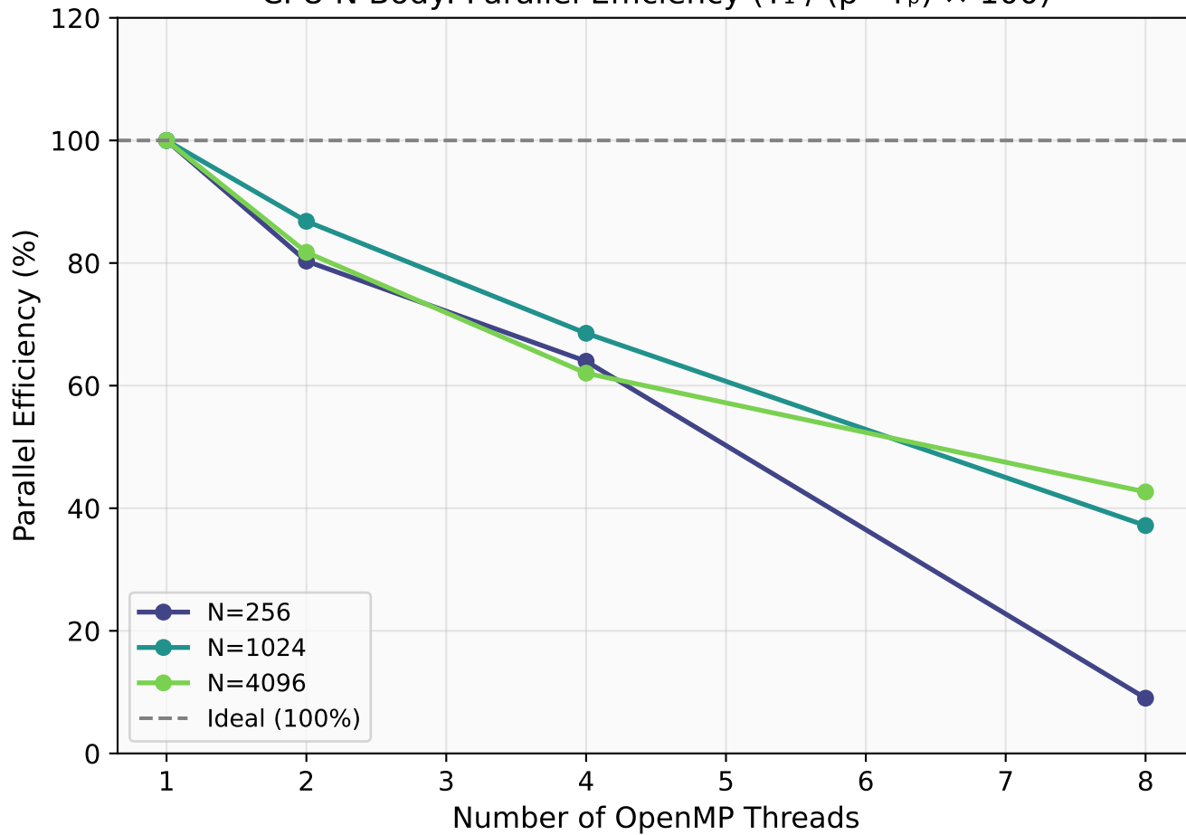
CPU N-Body: Parallel Efficiency ( T_1 / (p \cdot T_p) \times 100 )
