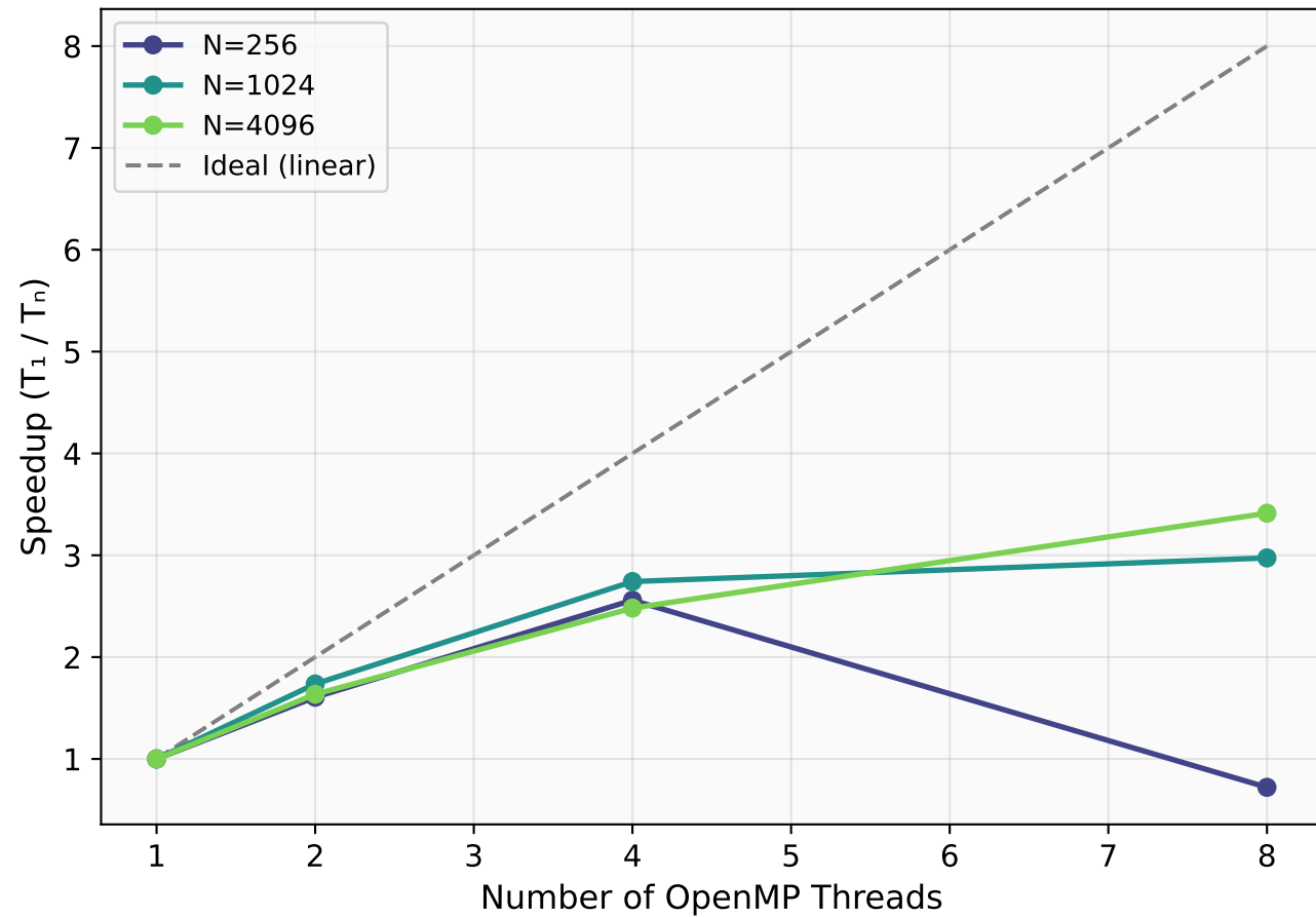
Parallel Speedup
