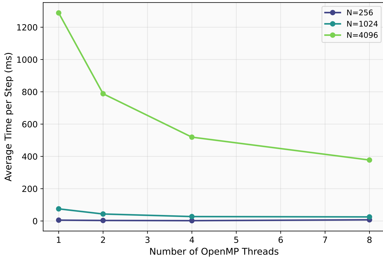
Execution Time vs Threads
