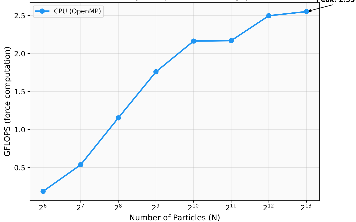
CPU N-Body: Computational Throughput
