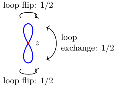
Figure 3. Figure-eight vacuum bubble: two loops joined at a vertex.
