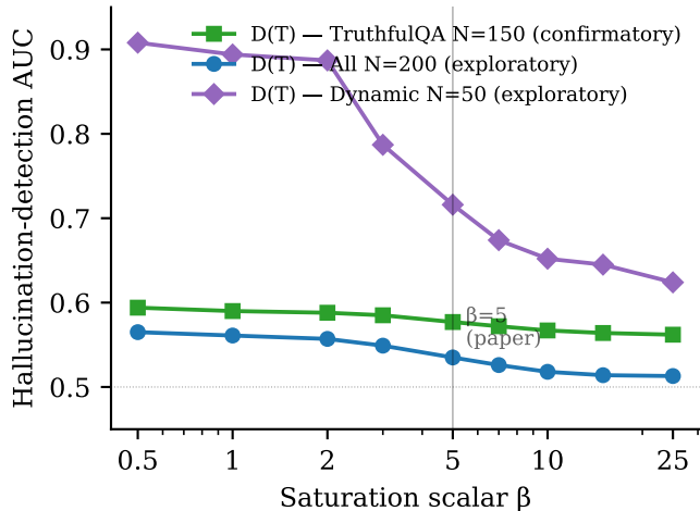
(a) Discriminative power vs. \beta
