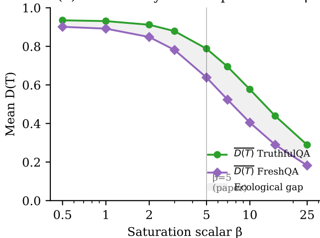
(b) Static-vs-Dynamic separation vs. \beta
