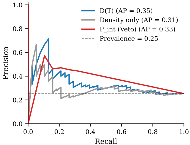
(b) Precision-Recall — reference-grounded
