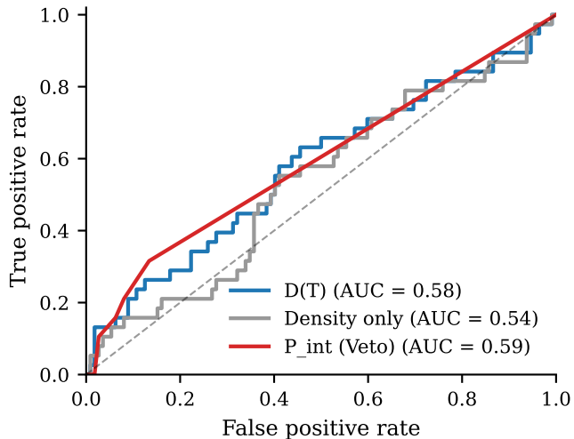
(a) ROC — reference-grounded TruthfulQA
