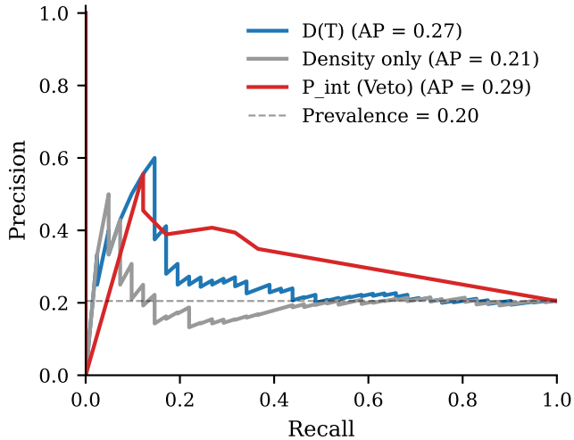
(b) Precision-Recall
