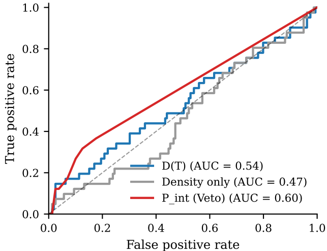
(a) ROC — hallucination detection
