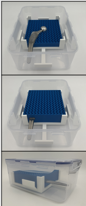
Hip Implant in Gyroid Lattice
