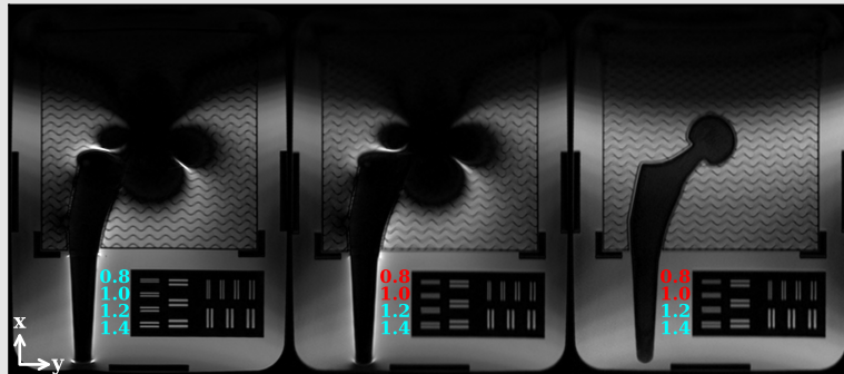
Metal Implant VAT-Off
