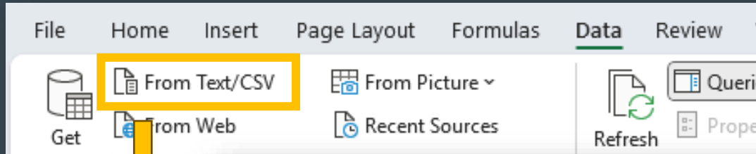
Computer_products_Sales(needs cleanup).csv
