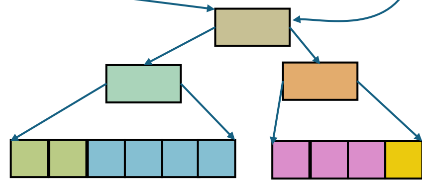
Tree- Based
