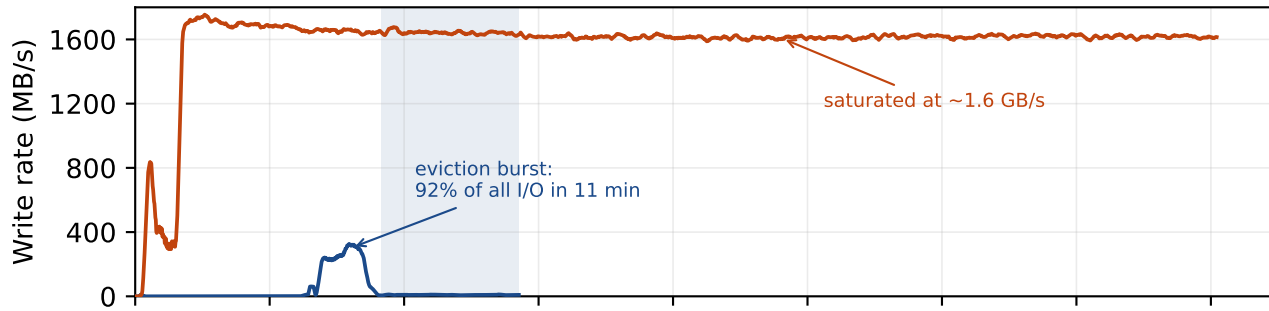
Disk write volume, update workload on graph500-24 (800 GiB cache, WAL off, no periodic checkpoint)
