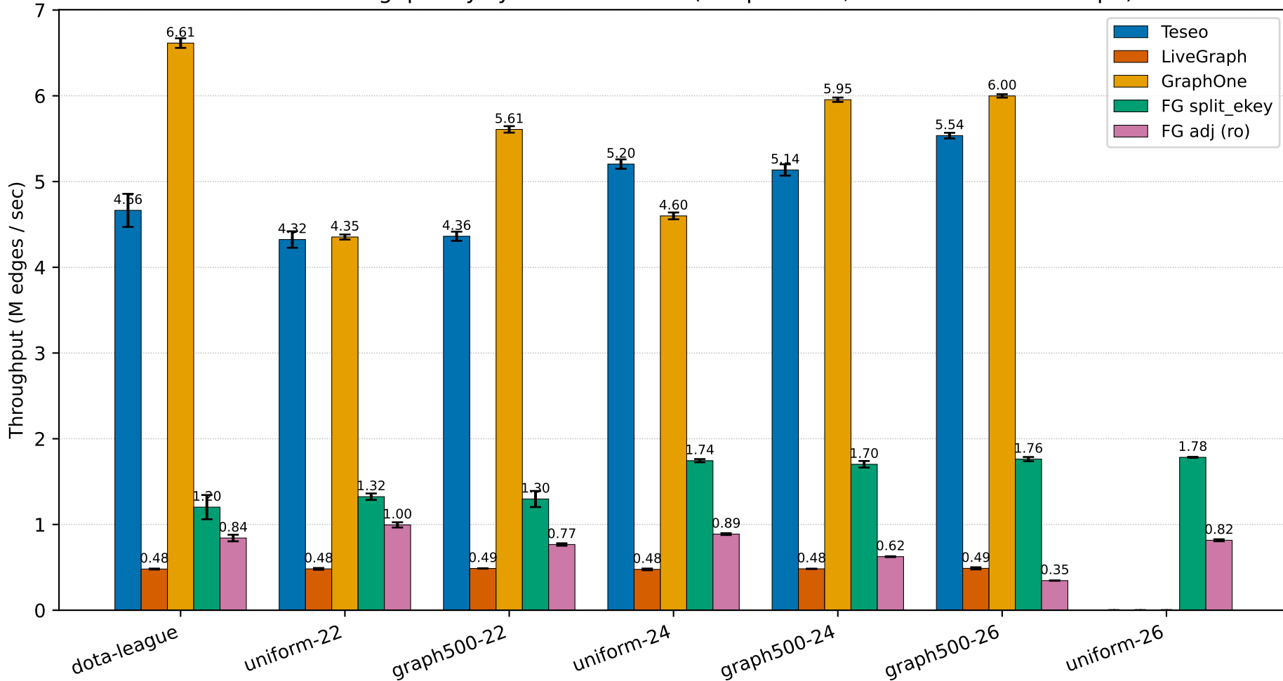
Insertion throughput by system × dataset (5-rep means; revert-state FlexoGraph)
