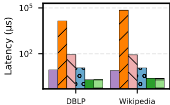
(c) Delete Edge
